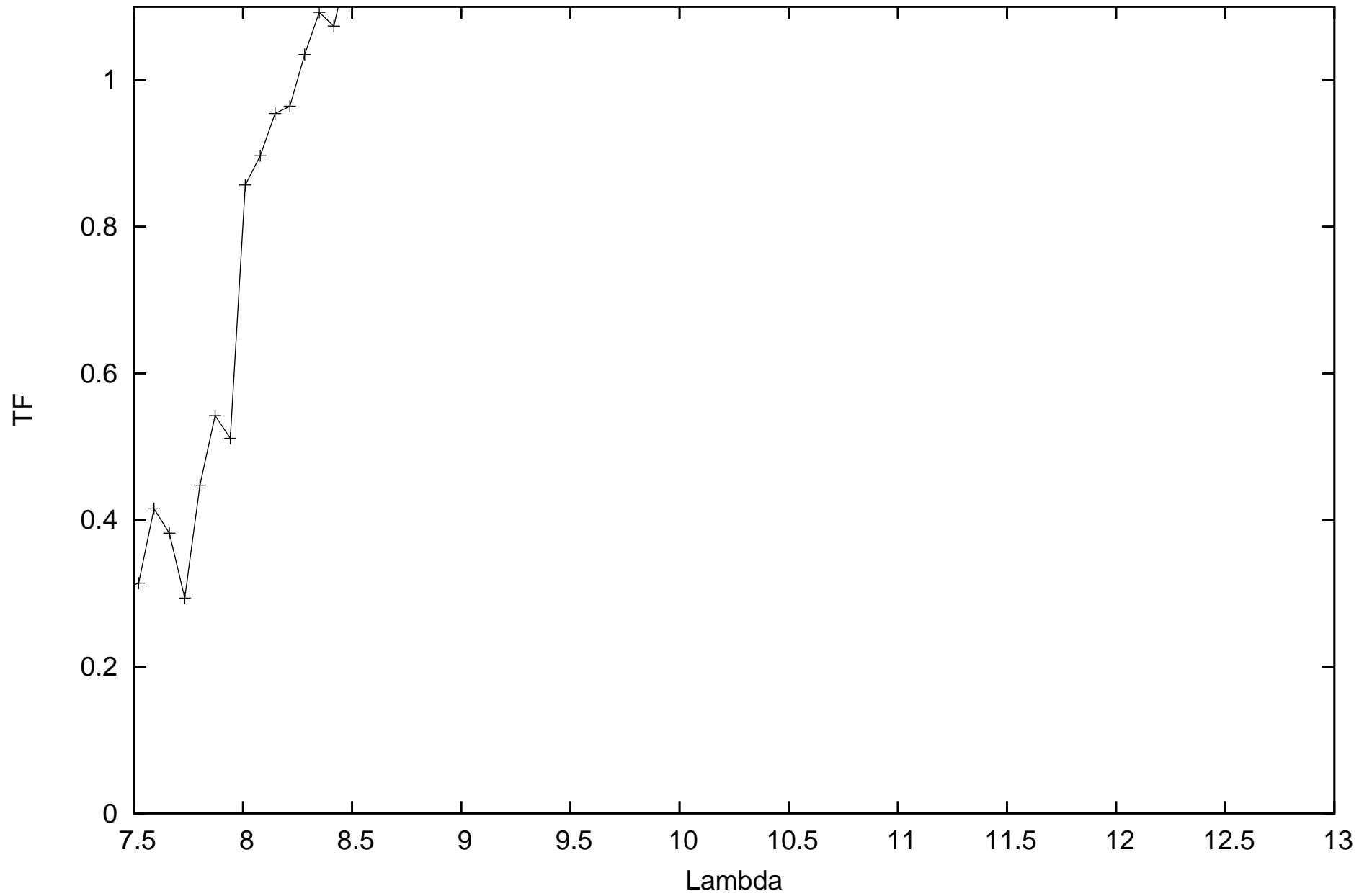
calHIP52447_flux3.85043_diam0.727197_r.MIDI.2011-03-22T00_22_57.000_U3U4
