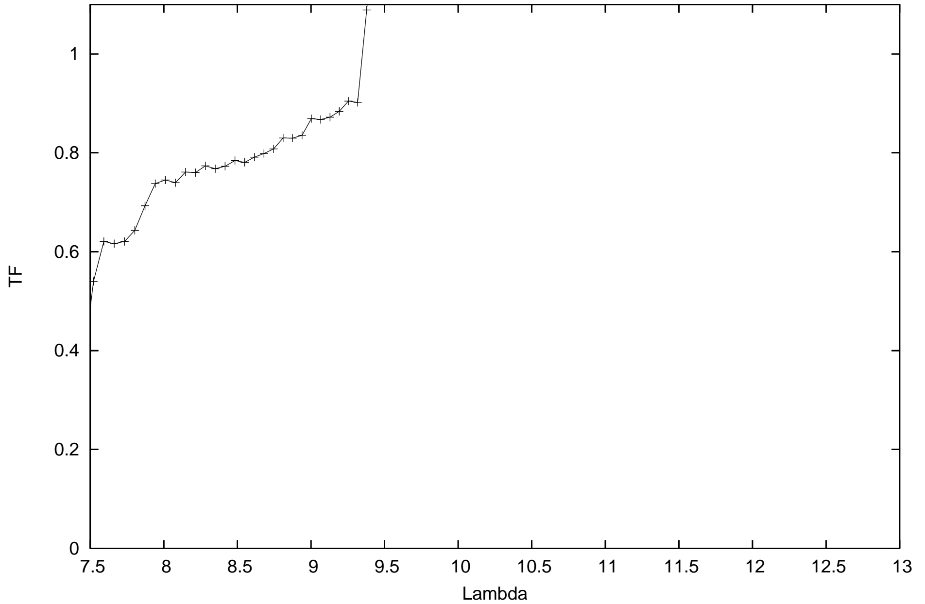
calHIP53151_flux2.90314_diam1.236103_r.MIDI.2011-03-20T04_46_40.000_U2U3
