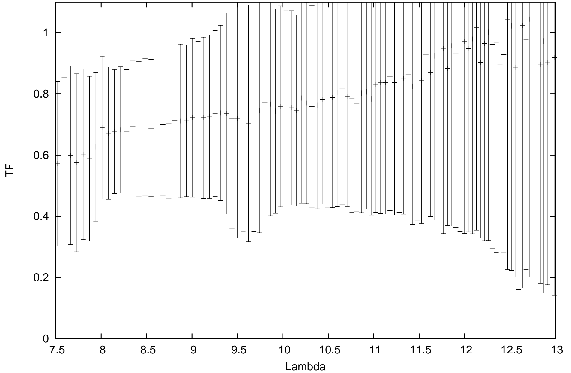
calHIP53151_flux2.90314_diam1.236103_r.MIDI.2011-03-23T03_02_00.000_U2U3
