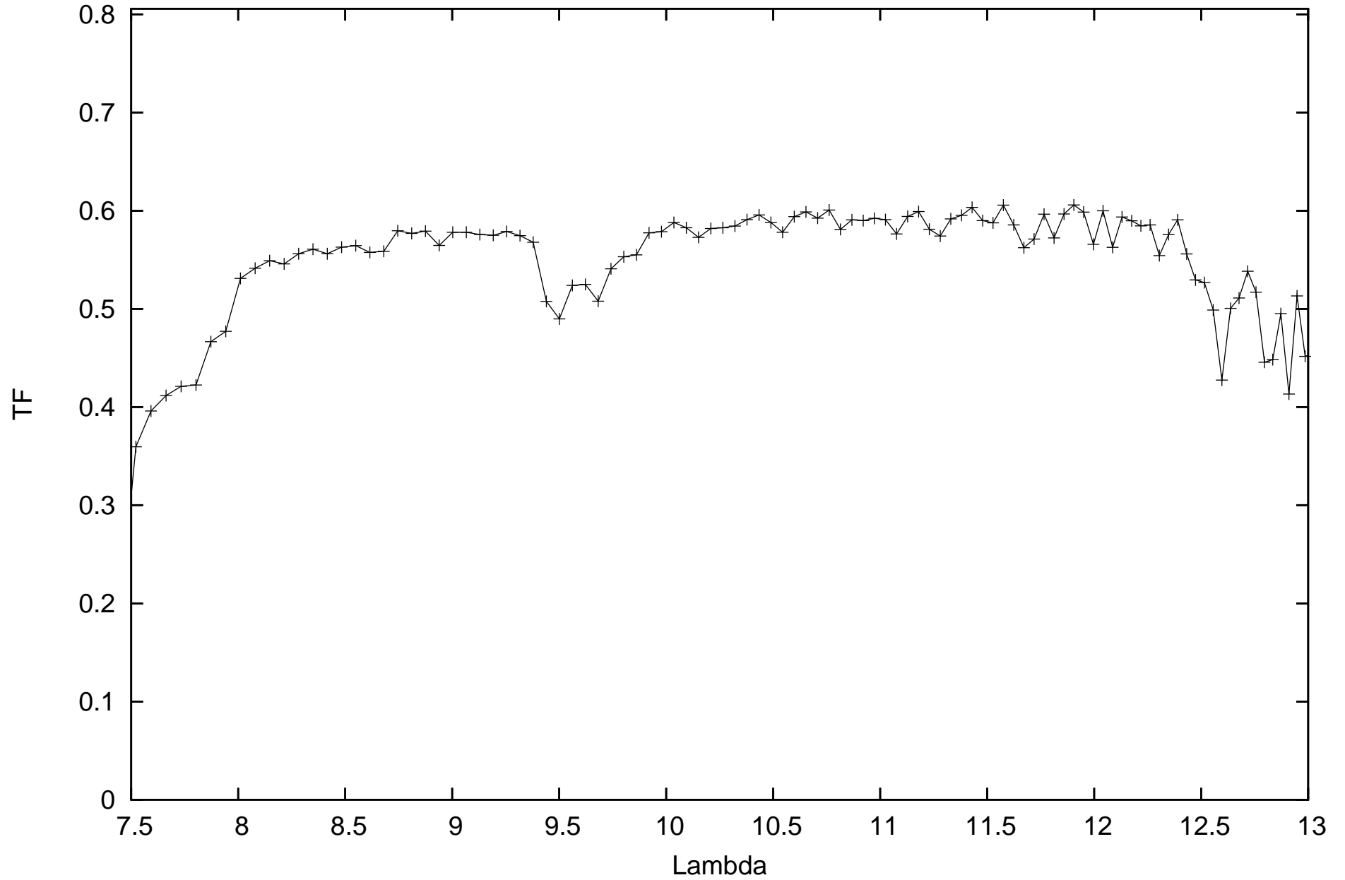
calHIP53151_flux2.90314_diam1.236103_r.MIDI.2011-03-24T03_12_15.000_U1U4
