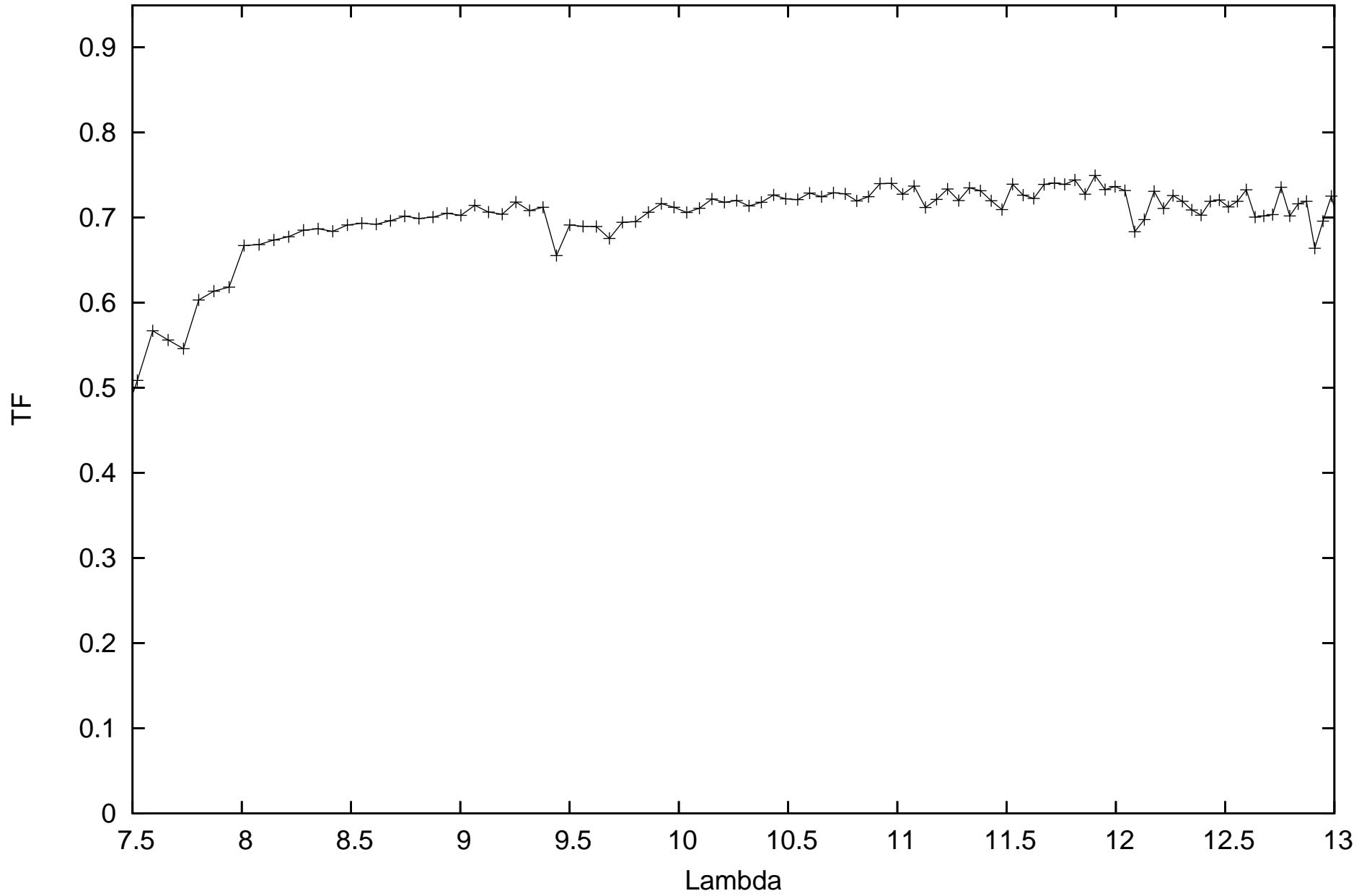
calHIP60172_flux2.02991_diam1.913526_r.MIDI.2011-03-23T07_56_29.000_U1U4
