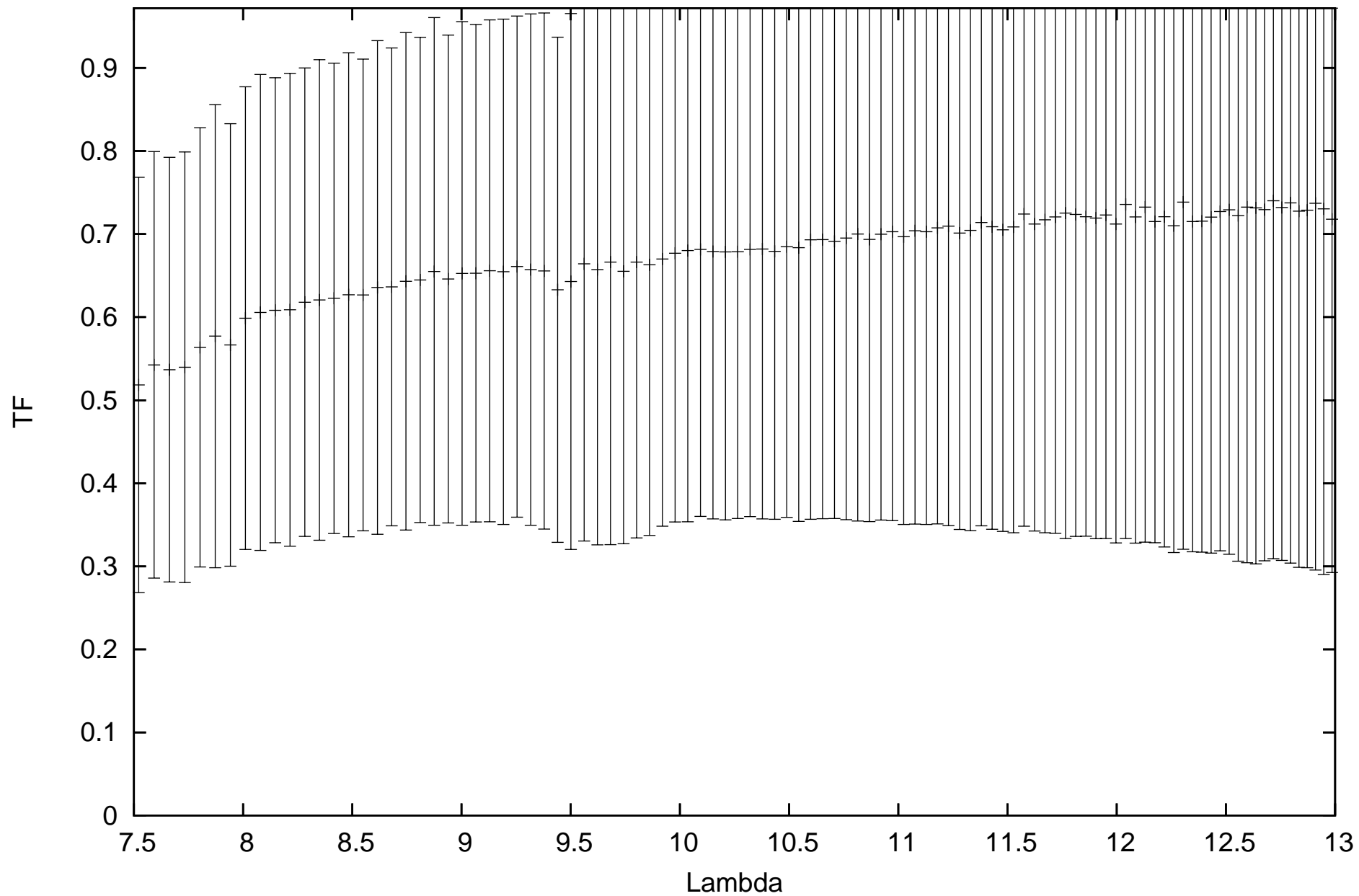
calHIP63066_flux1.00467_diam3.16_r.MIDI.2011-04-18T01_15_19.000_U2U4
