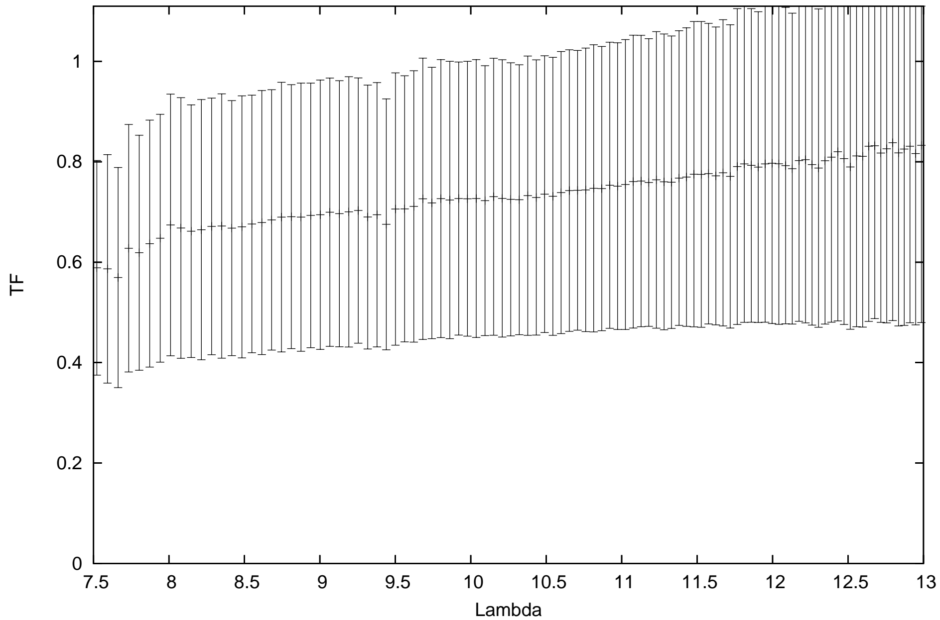
calHIP68895_flux0.550435_diam3.55_r.MIDI.2011-04-15T02_29_35.000_U2U3
