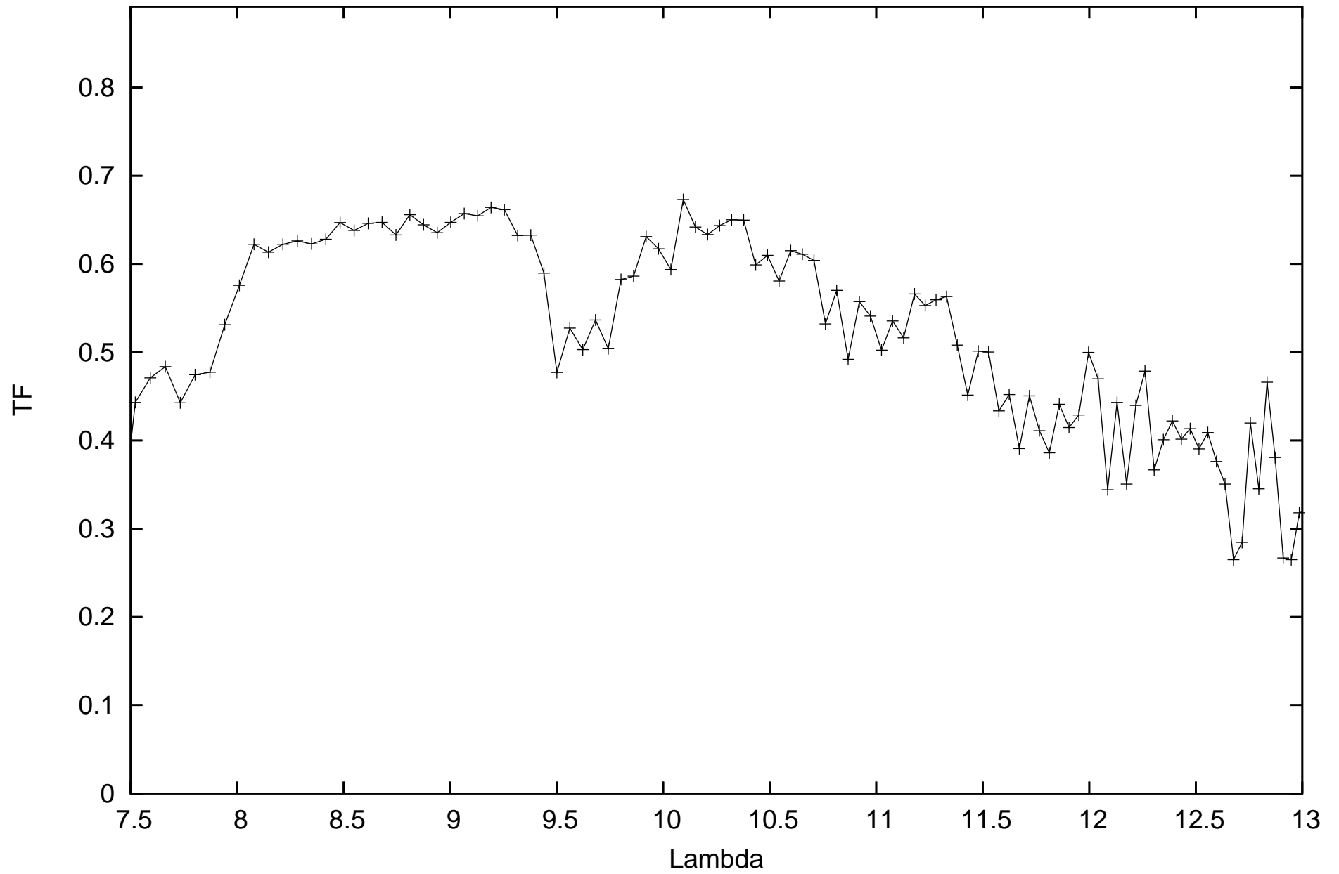
calHIP78870_flux3.70545_diam0.82654_r.MIDI.2011-04-18T07_14_33.000_U1U4
