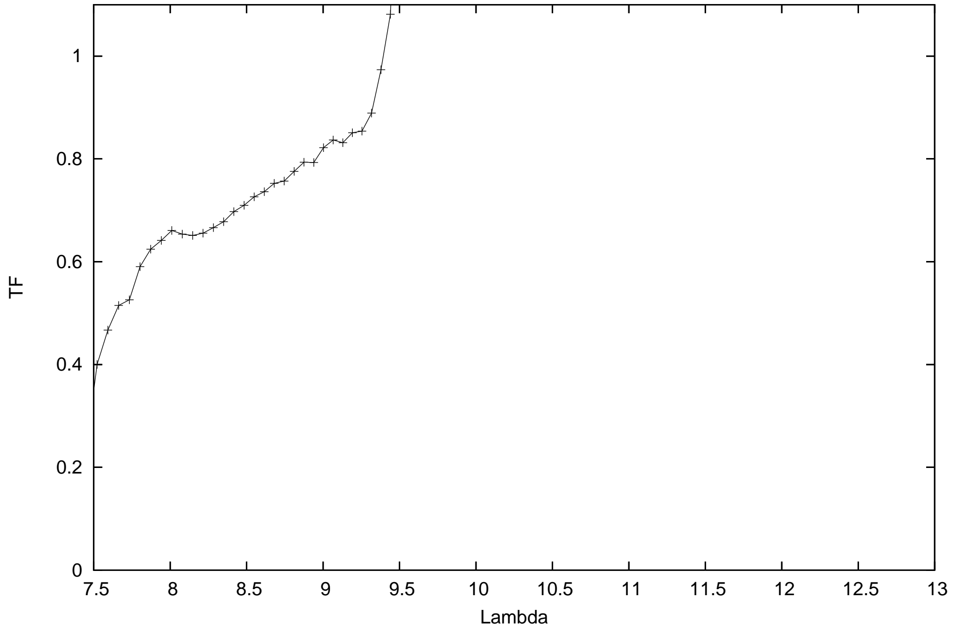
calHIP81616_flux2.5384_diam1.51919_r.MIDI.2011-03-20T06_01_50.000_U2U3
