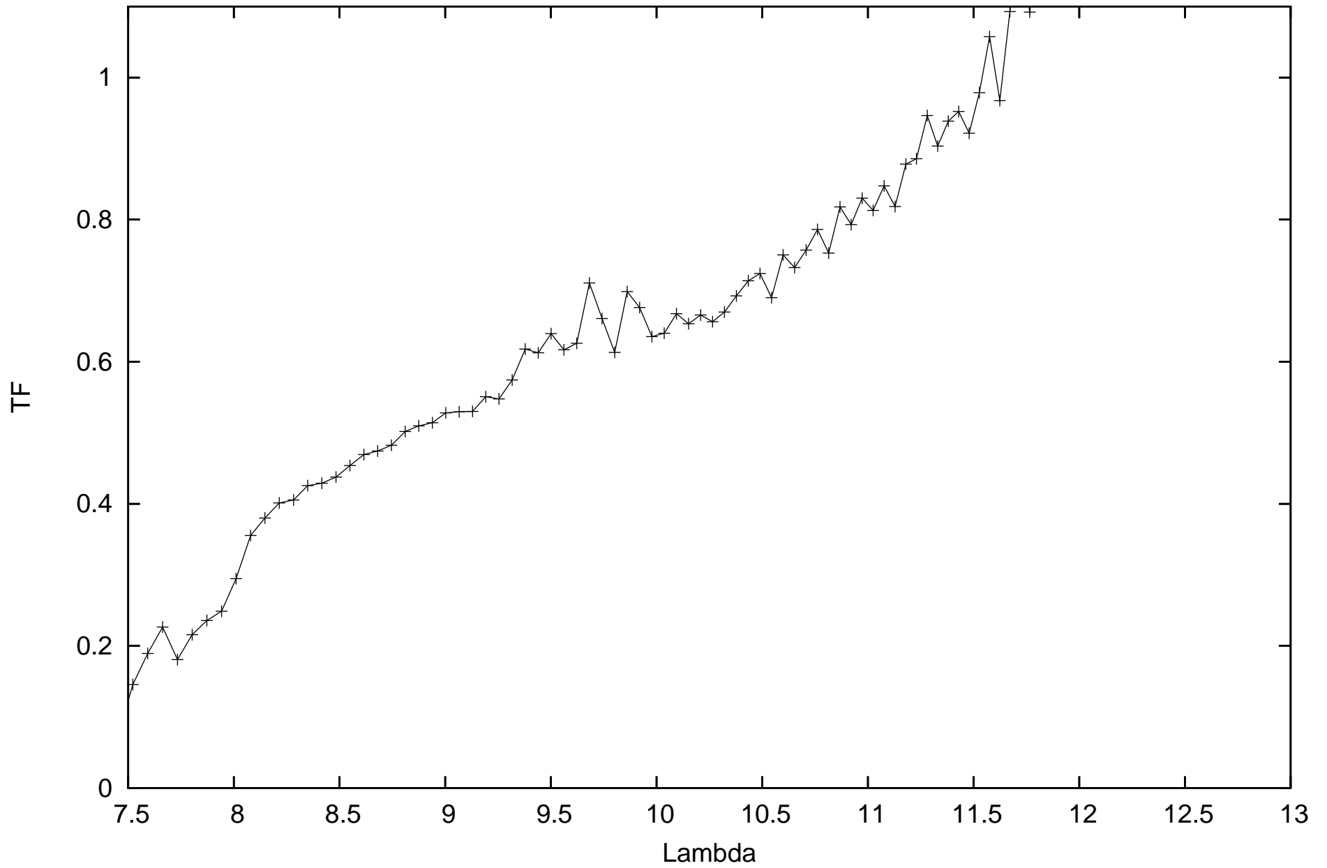
calHIP81616_flux2.5384_diam1.51919_r.MIDI.2011-04-13T04_16_09.000_U2U3
