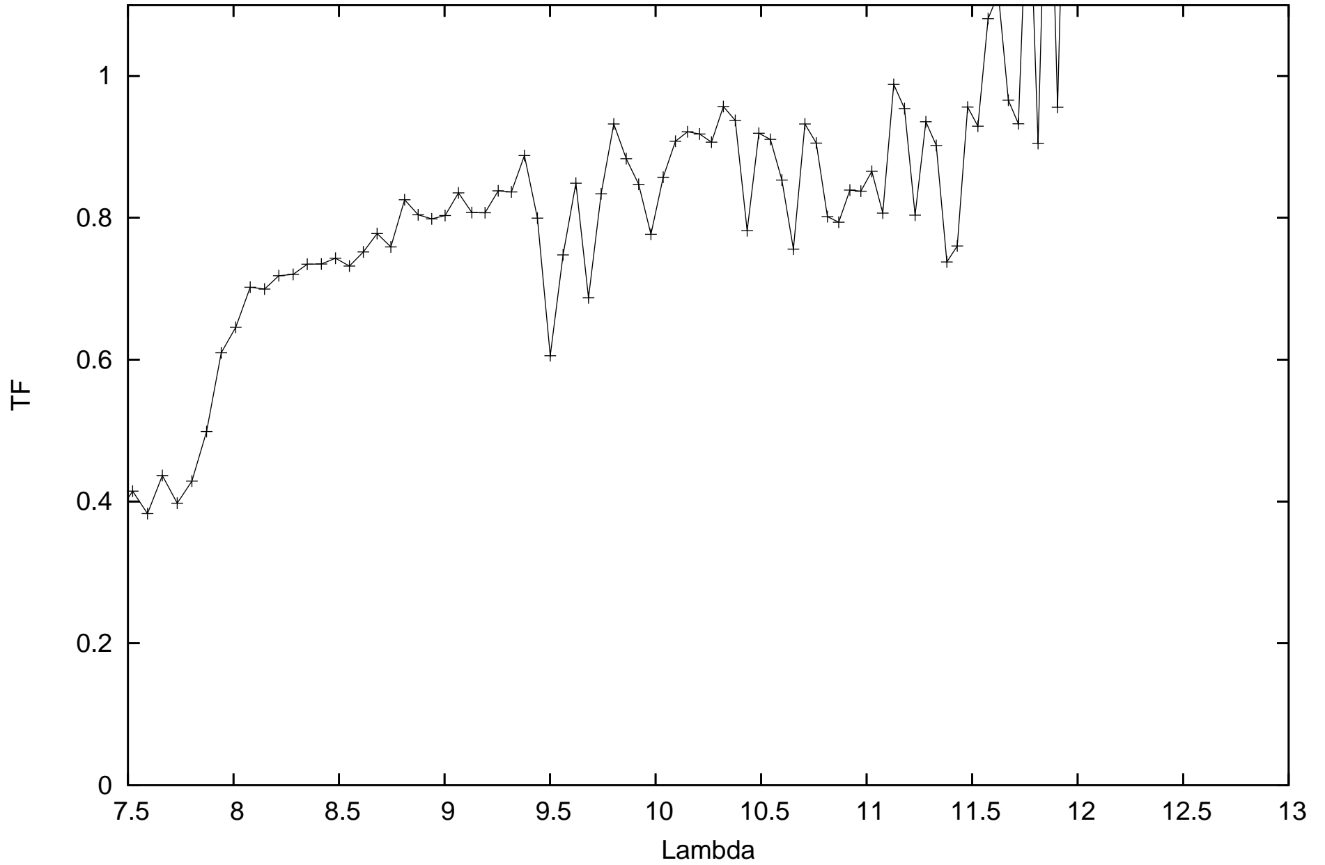
calHIP81731_flux3.80301_diam0.768588_r.MIDI.2011-05-14T05_32_54.000_U3U4
