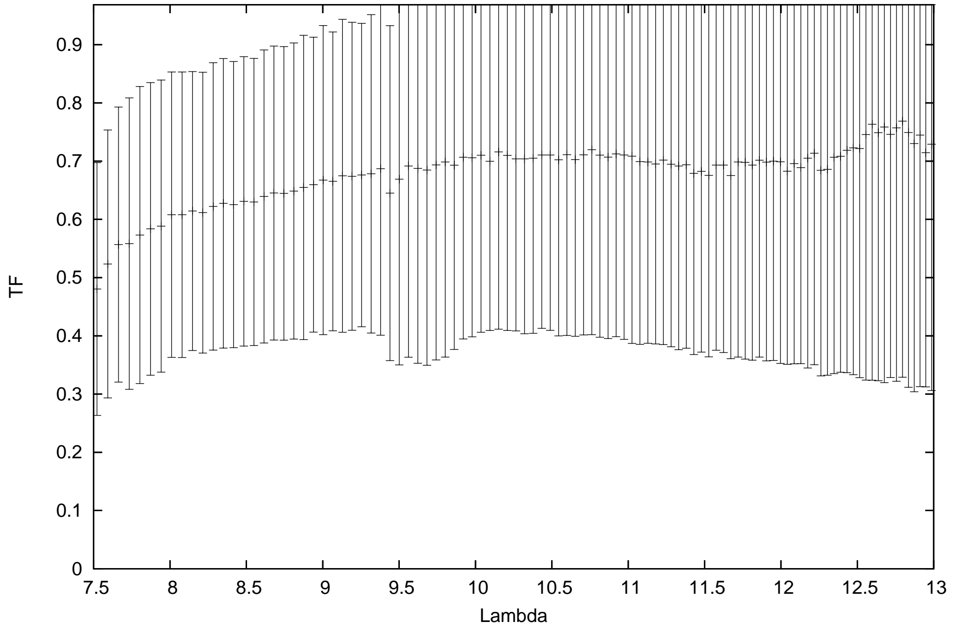
calHIP82273_flux-1.42243_diam8.91_r.MIDI.2011-04-23T04_56_30.000_K011
