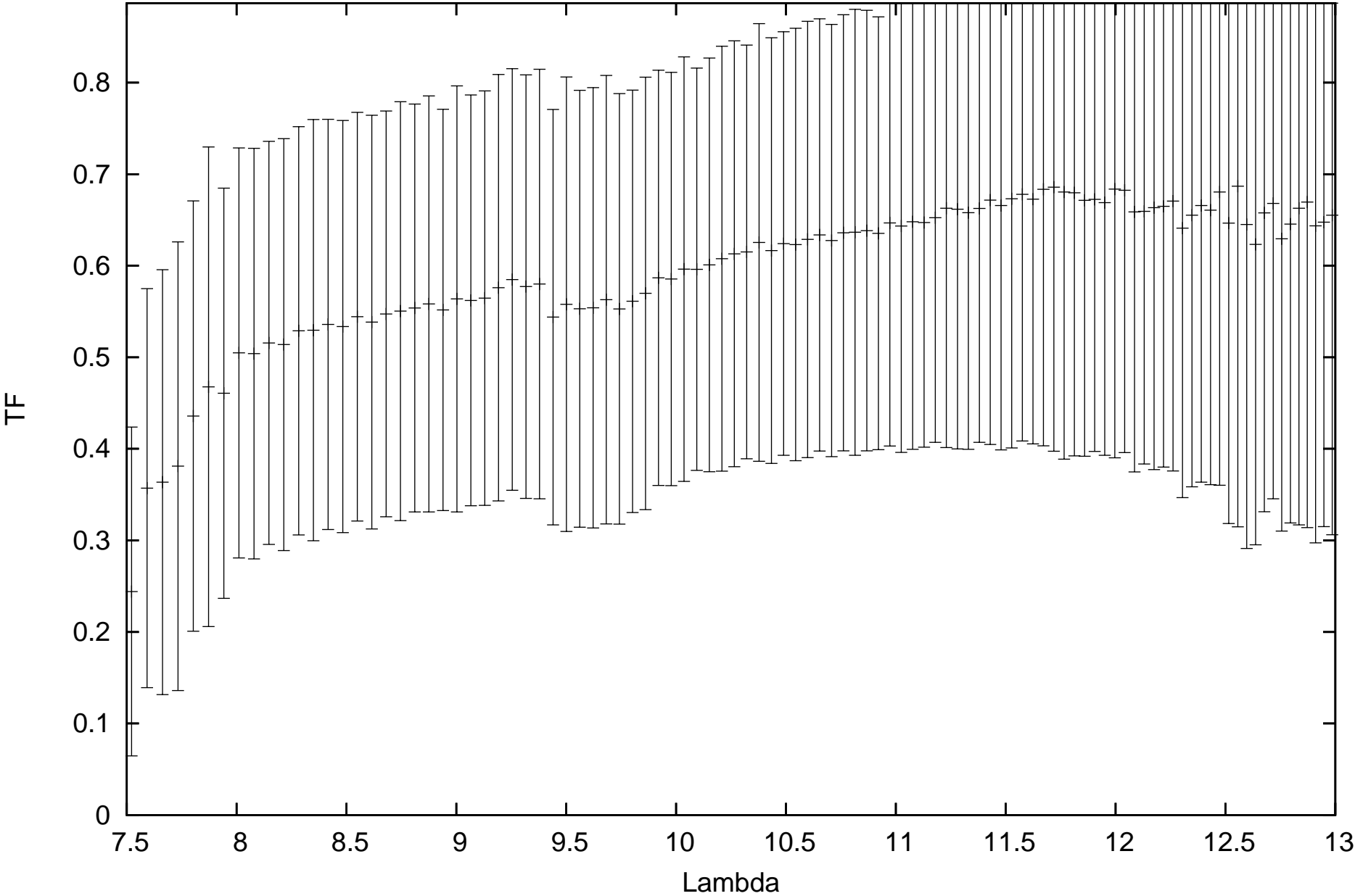
calHIP82273_flux-1.42243_diam8.91_r.MIDI.2011-05-30T09_42_36.000_D0G1
