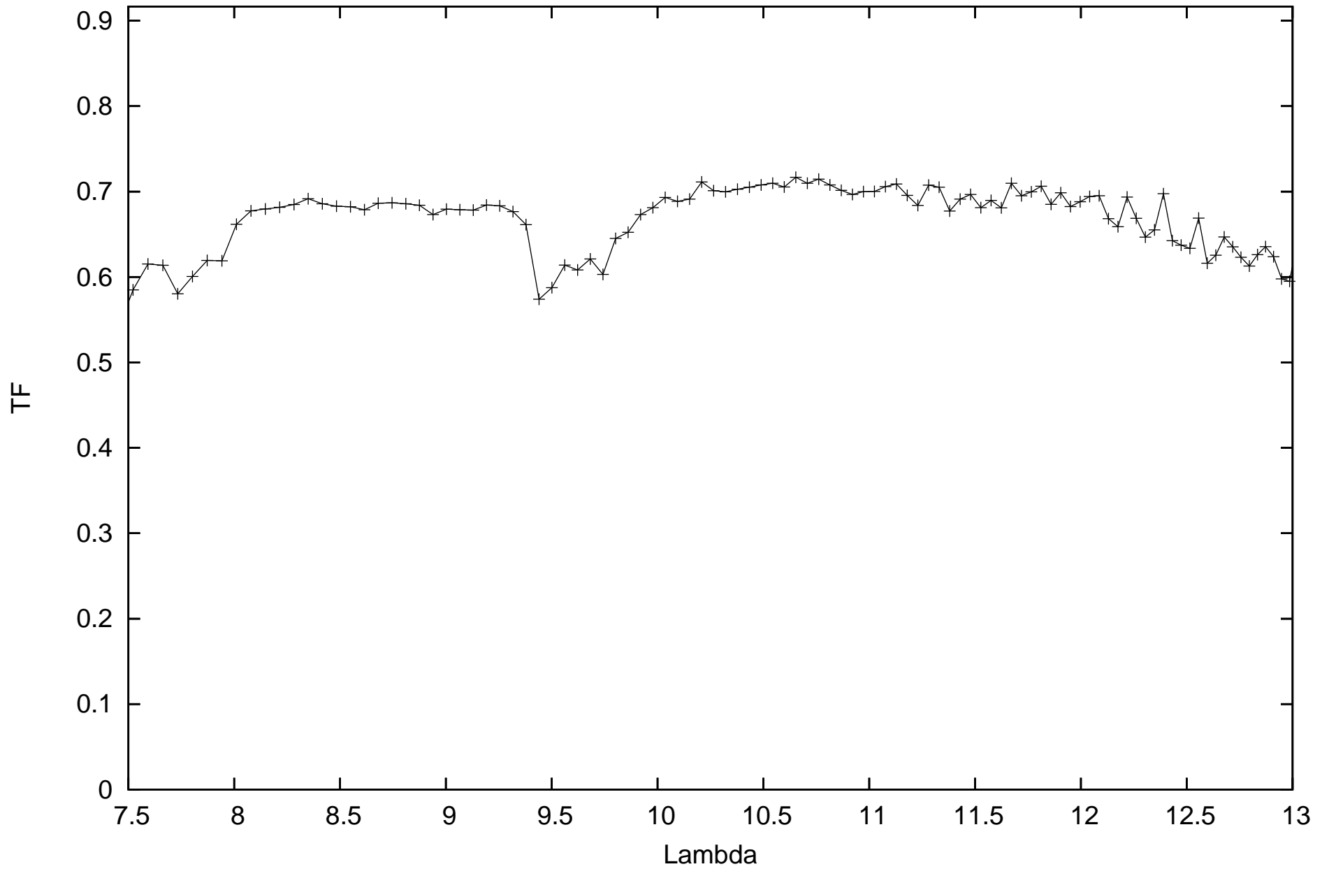
calHIP82273_flux-1.42243_diam8.91_r.MIDI.2011-08-10T03_17_22.000_D0A1
