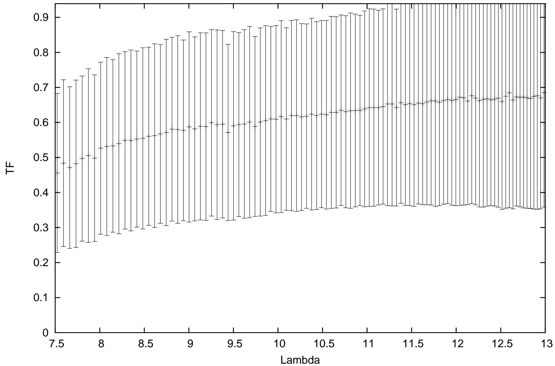
calHIP82729_flux0.277058_diam4.09_r.MIDI.2011-04-14T06_02_59.000_U1U2
