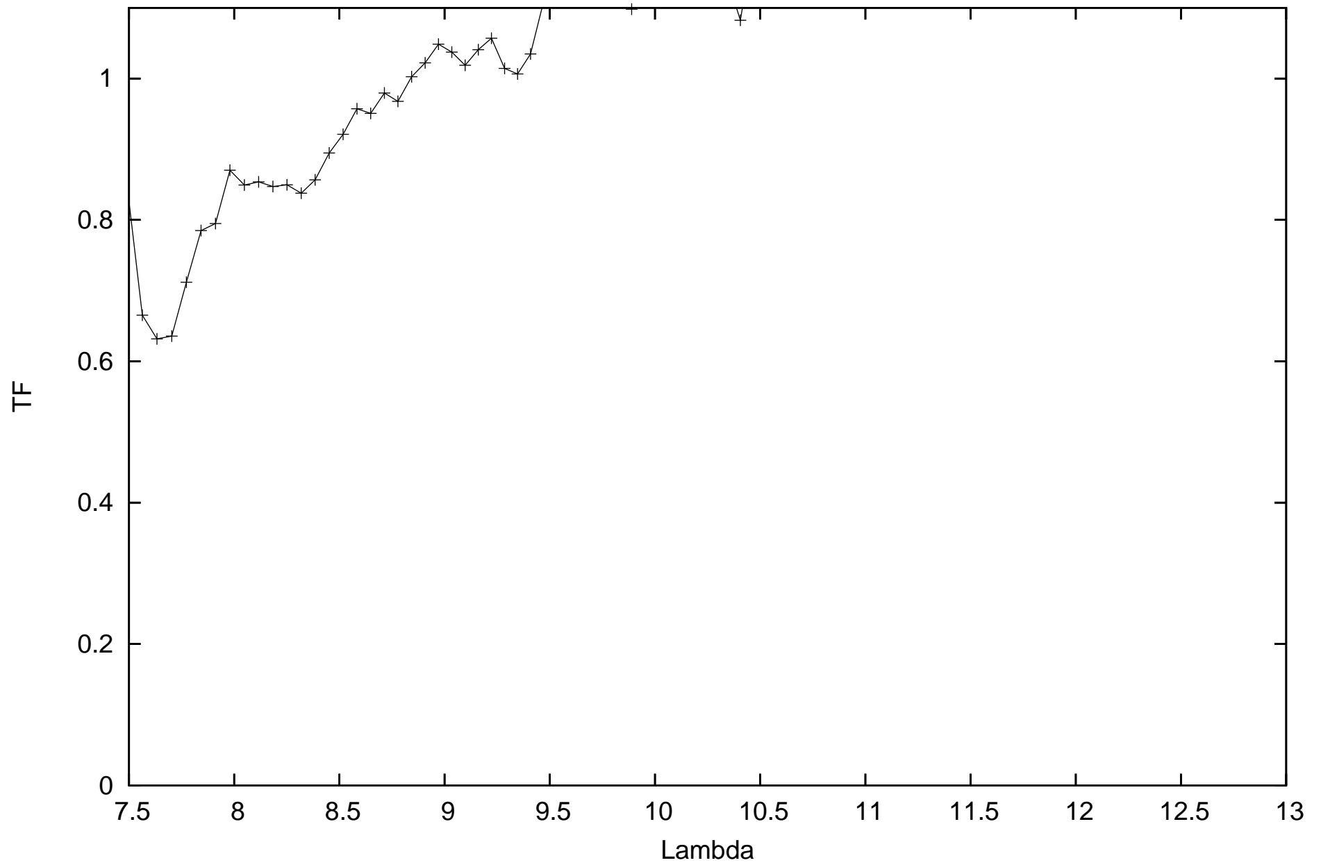
calHIP83081_flux-0.81238_diam6.88_r.MIDI.2011-06-11T00_42_20.945_B2A1
