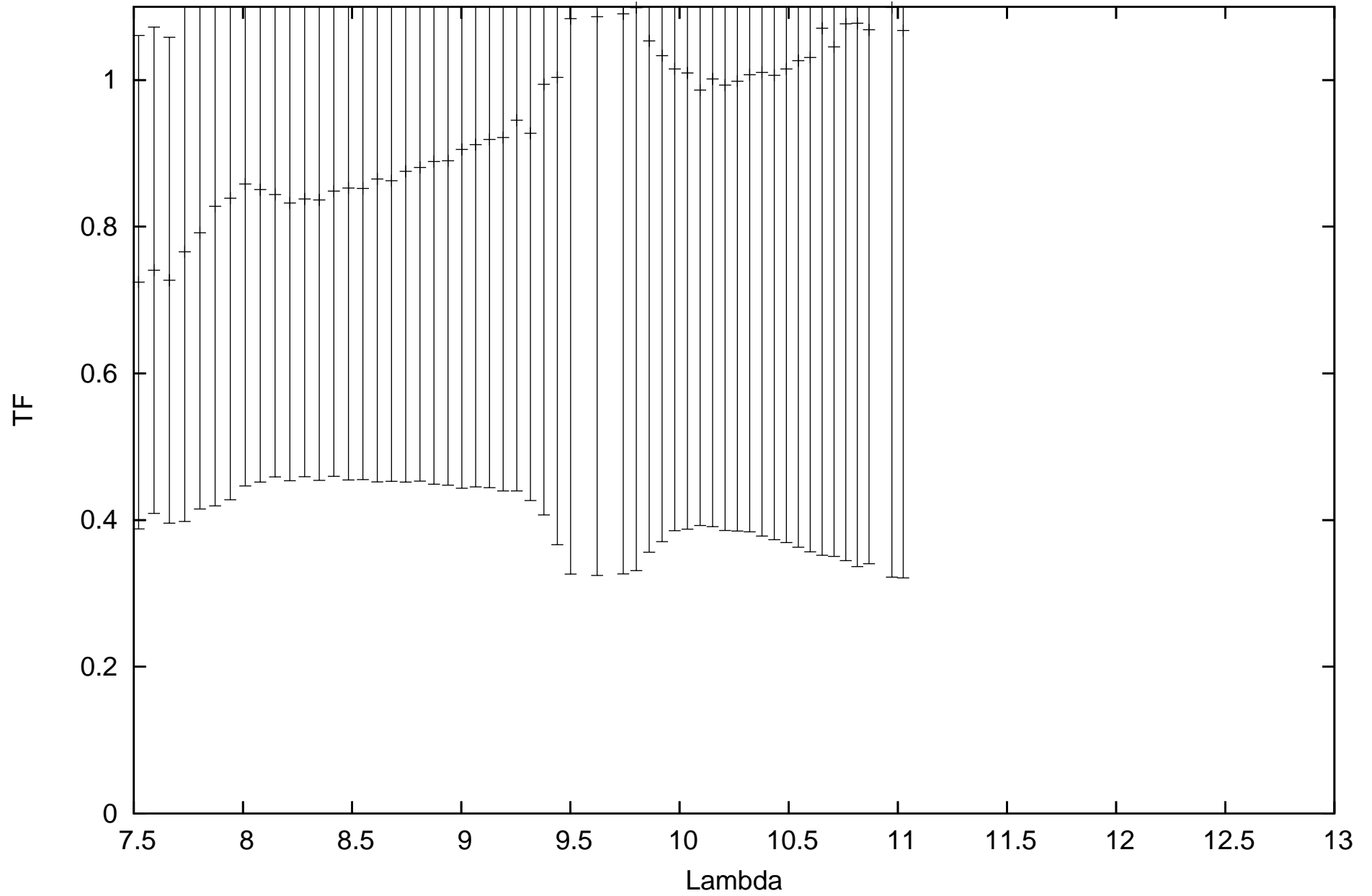
calHIP89931_flux-0.511_diam5.87_r.MIDI.2011-04-27T09_53_31.000_G111
