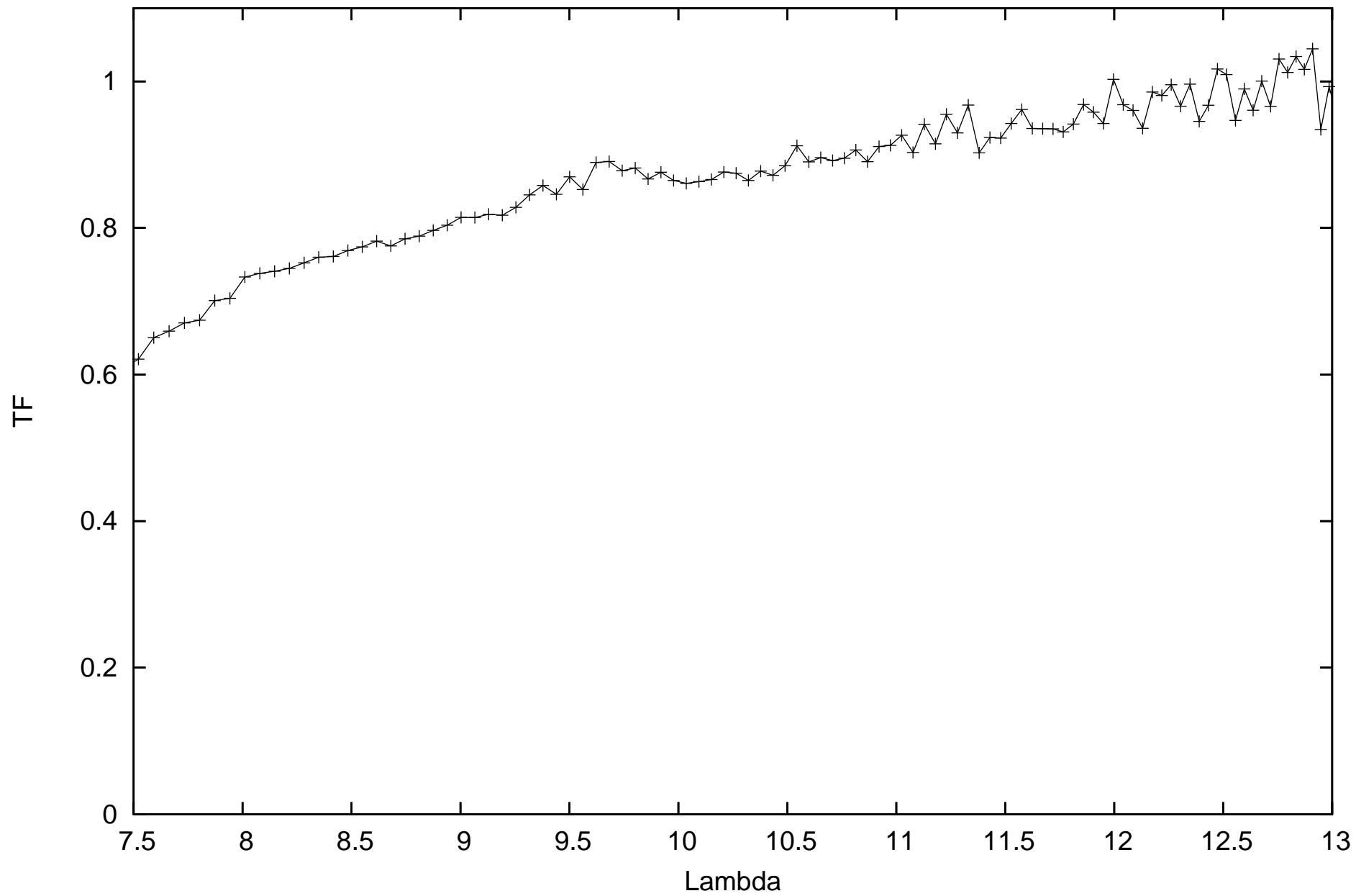
calHIP89931_flux-0.511_diam5.87_r.MIDI.2011-05-02T07_00_03.000_G111
