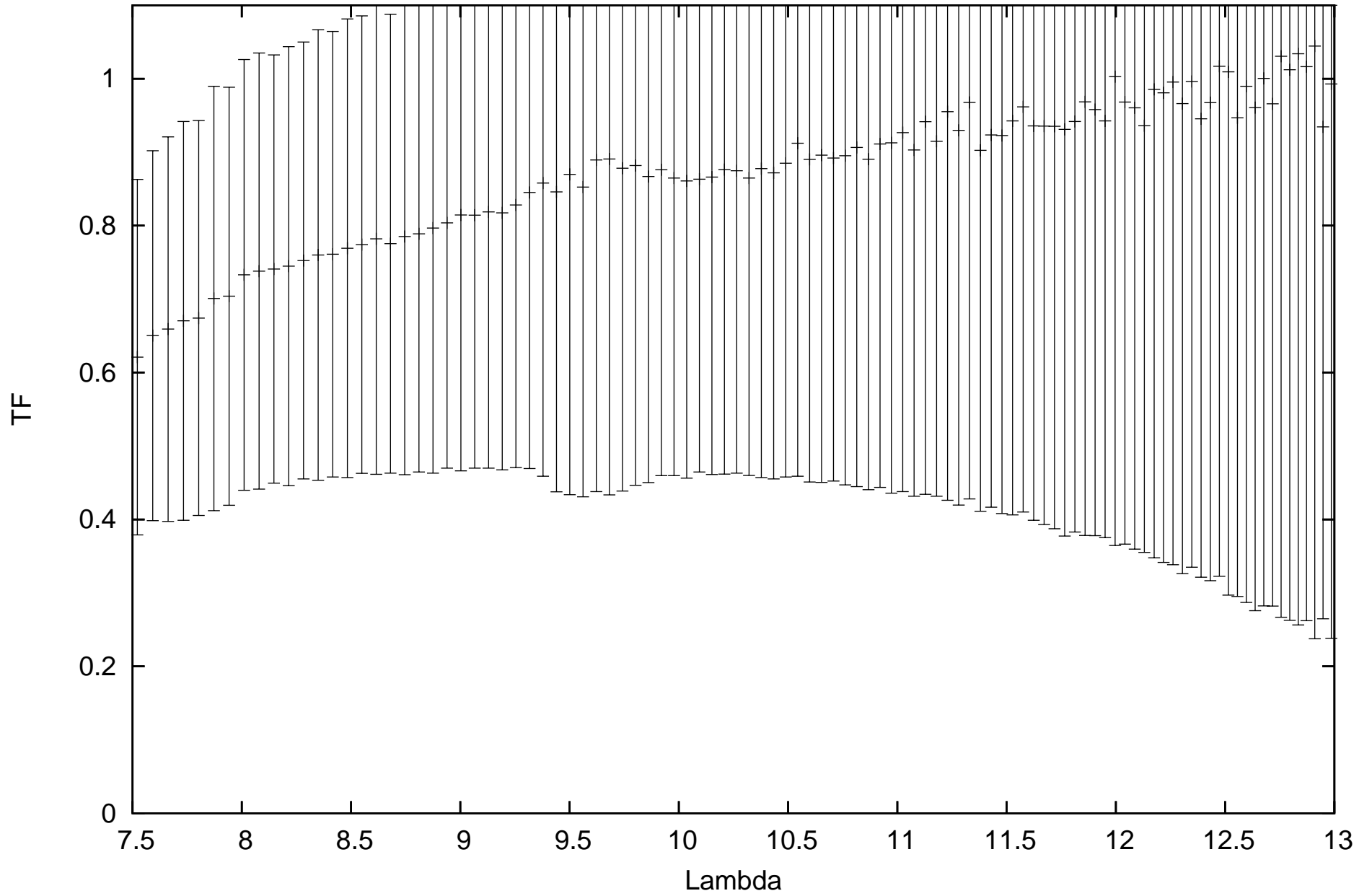
calHIP89931_flux-0.511_diam5.87_r.MIDI.2011-05-02T07_00_03.000_G111
