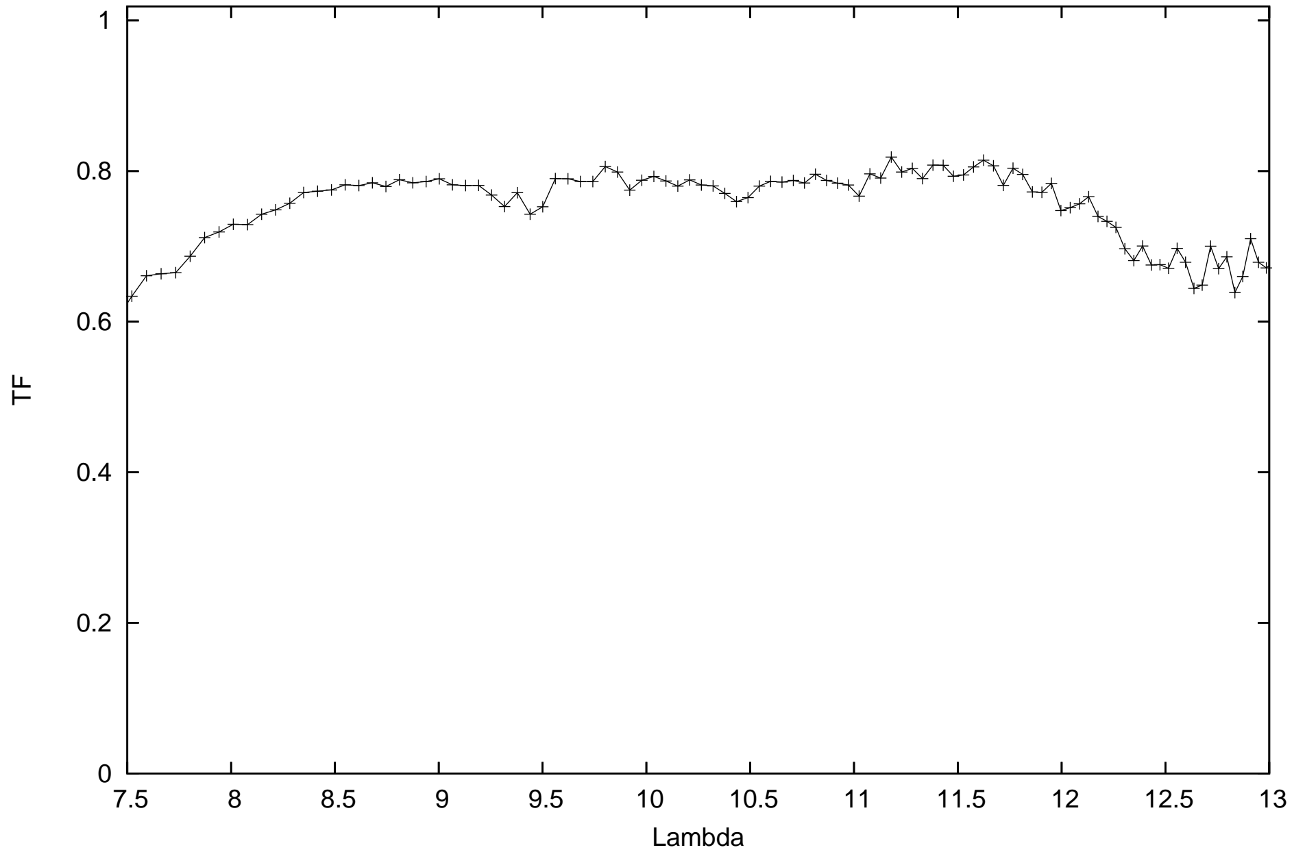
calHIP89931_flux-0.511_diam5.87_r.MIDI.2011-07-26T05_38_29.000_K011
