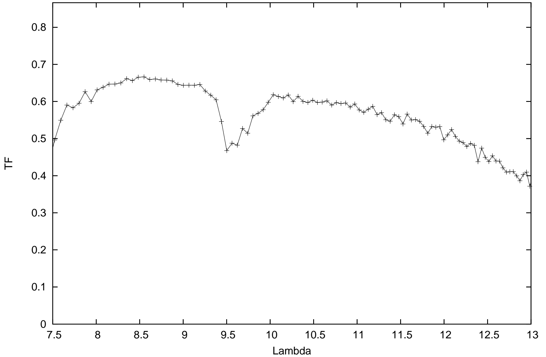
calHIP89931_flux-0.511_diam5.87_r.MIDI.2011-07-26T06_24_12.000_G111
