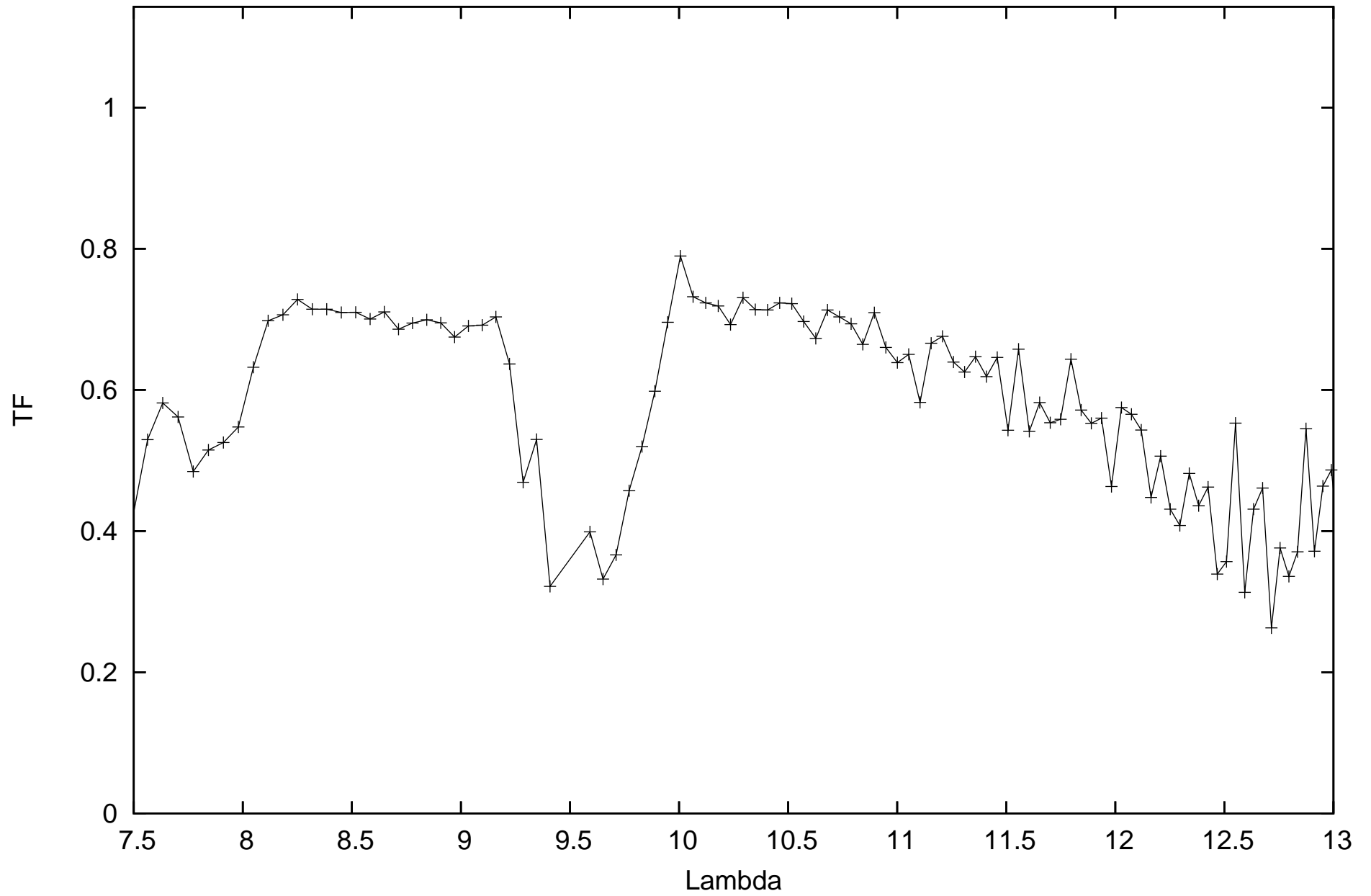
calHIP89931_flux-0.511_diam5.87_r.MIDI.2011-11-03T23_48_40.969_G111
