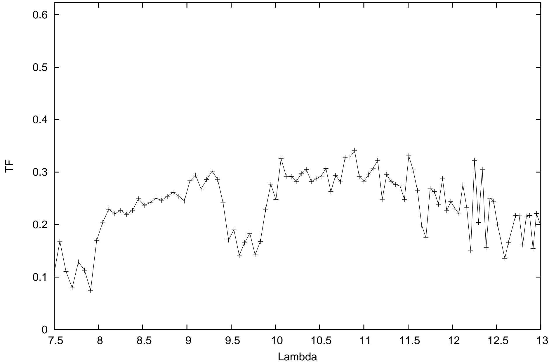
calHIP89931_flux-0.511_diam5.87_r.MIDI.2011-11-11T00_08_21.932_K011
