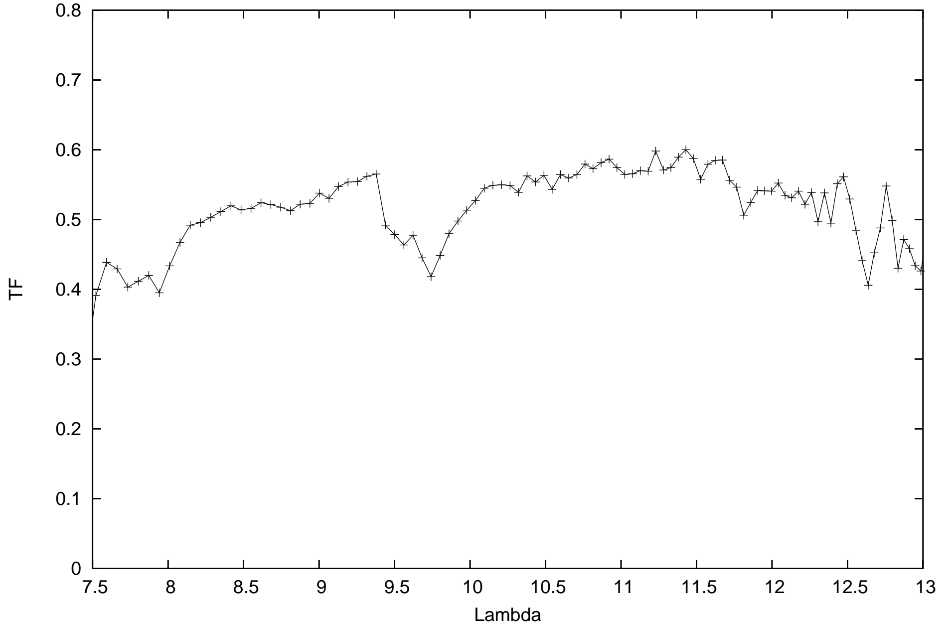
calHIP9884_flux-0.75397_diam7.42869_r.MIDI.2011-11-07T05_18_05.000_K0G1
