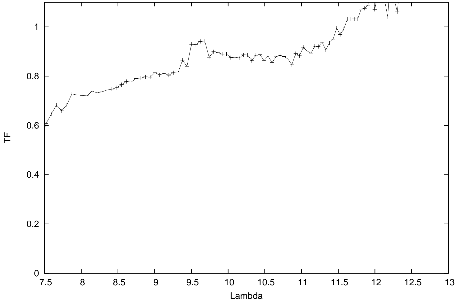
calHIP9884_flux-0.75397_diam7.42869_r.MIDI.2011-12-04T01_09_27.000_K0J3
