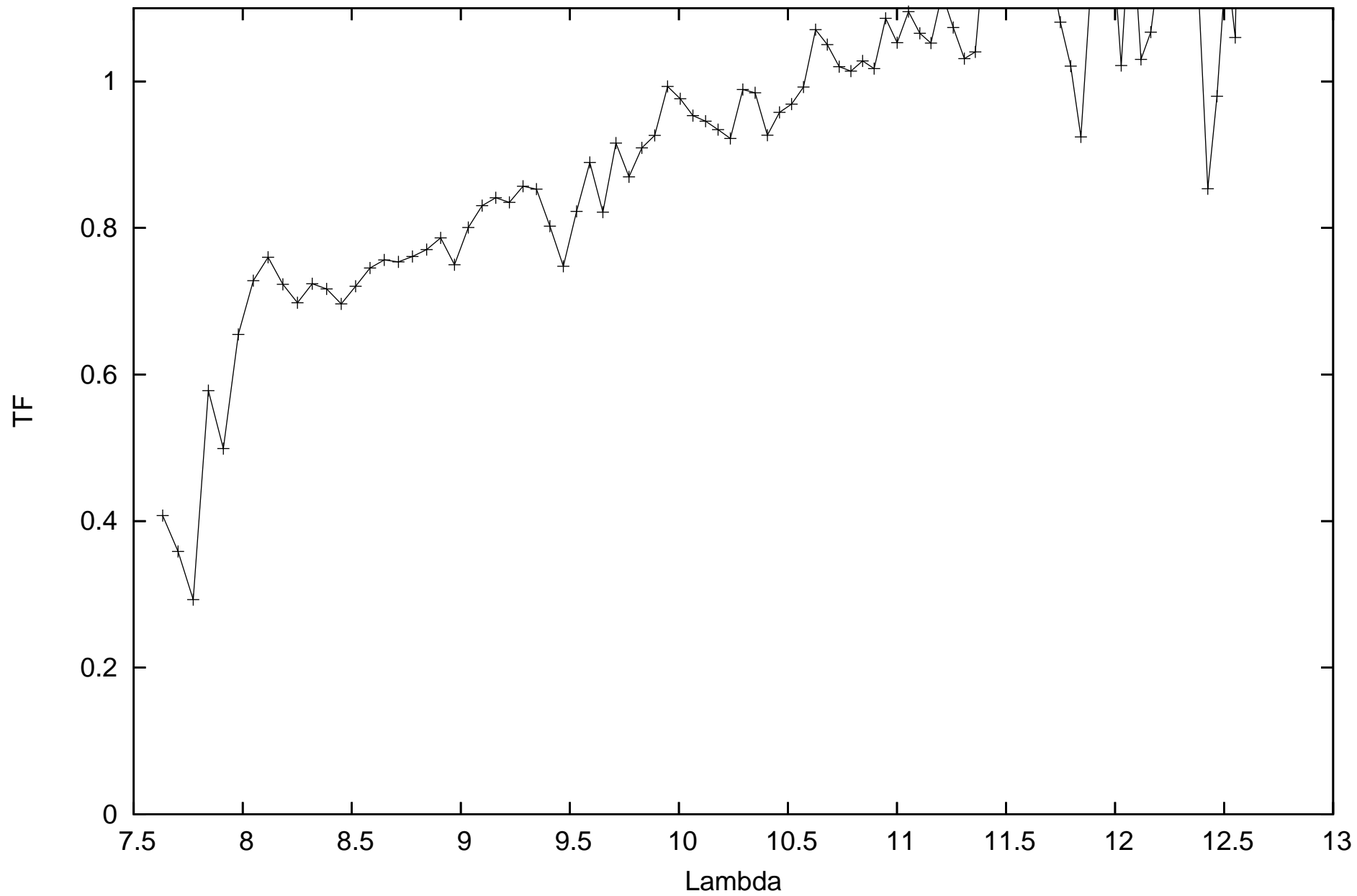
calHIP83081_flux-0.81238_diam6.88_r.MIDI.2012-01-26T09_08_28.105_D0C1
