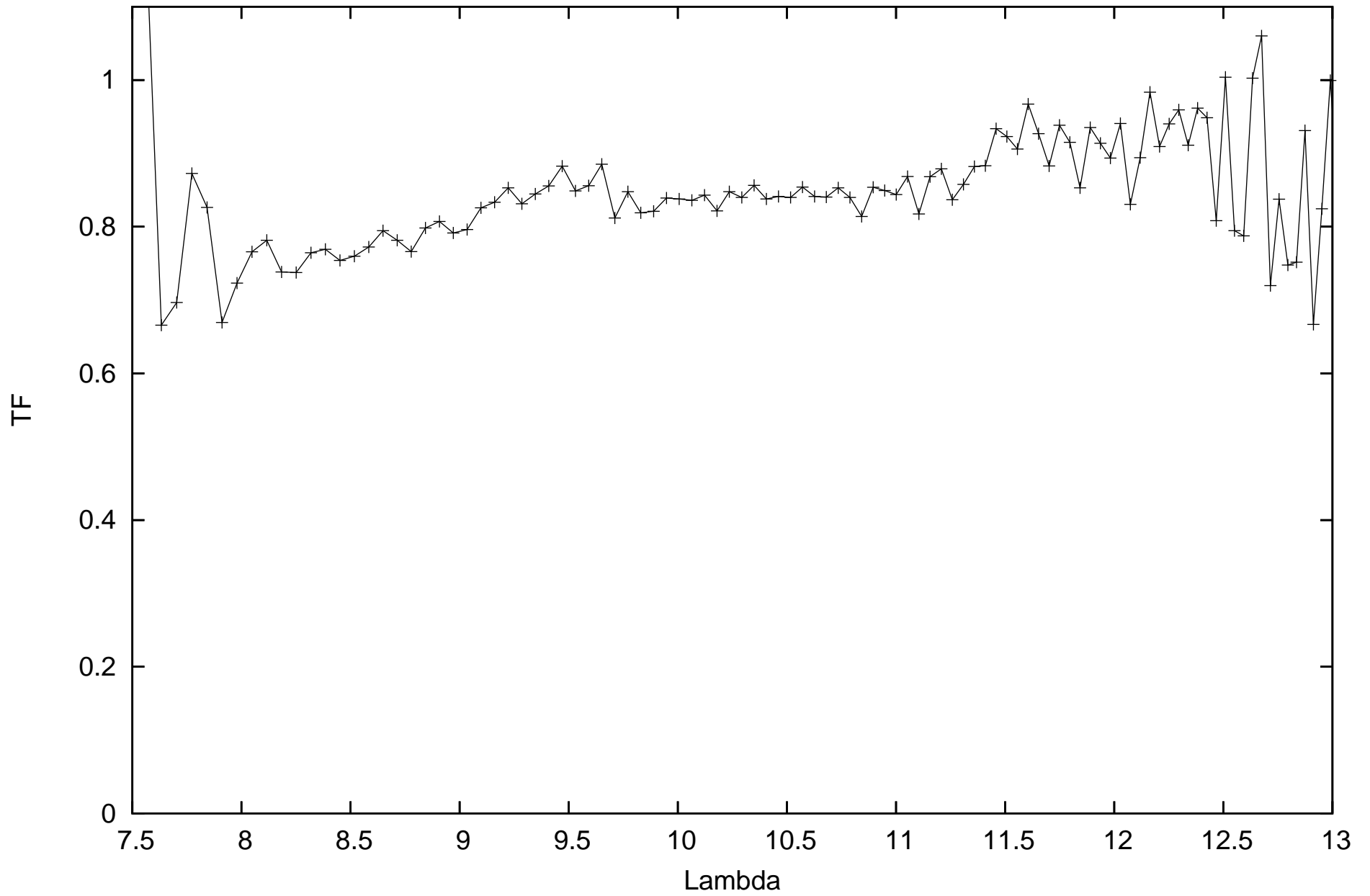
calHD81797_flux-1.49_diam9.14_r.MIDI.2012-01-28T04_17_43.970_C1B2
