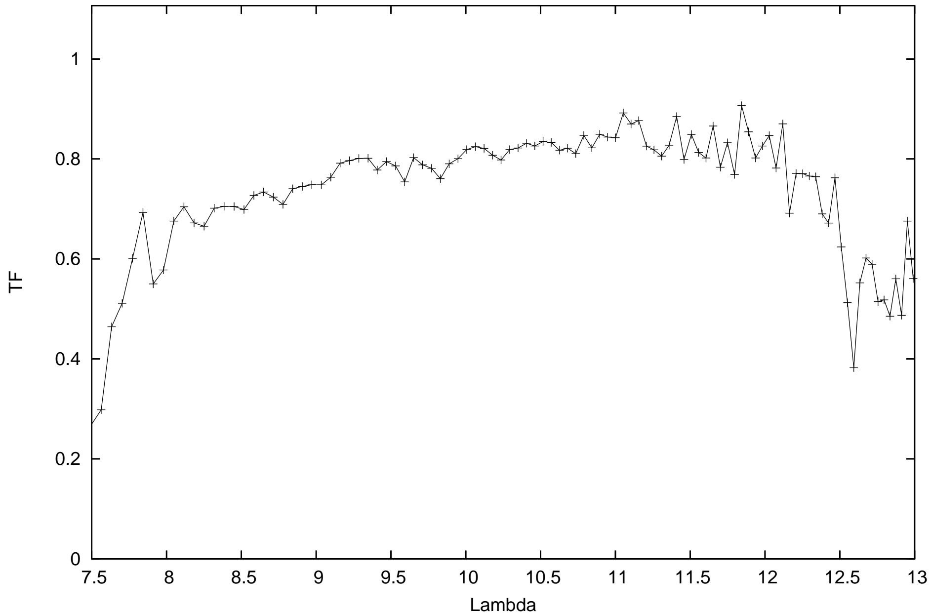
calHD81797_flux-1.49_diam9.14_r.MIDI.2012-01-28T05_32_54.135_B2A1
