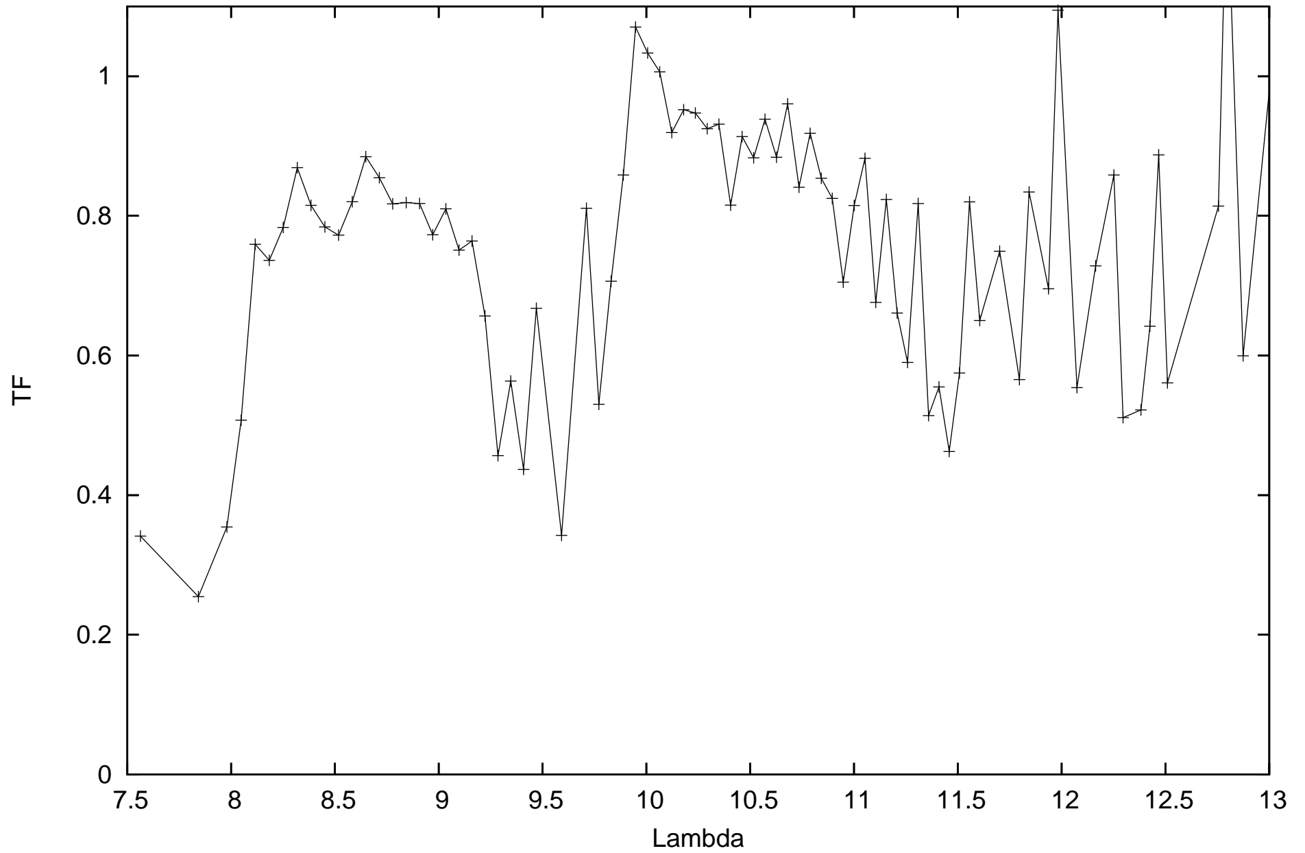
calHIP50371_flux-0.22962_diam5.18_r.MIDI.2012-01-29T02_14_03.939_D0B2
