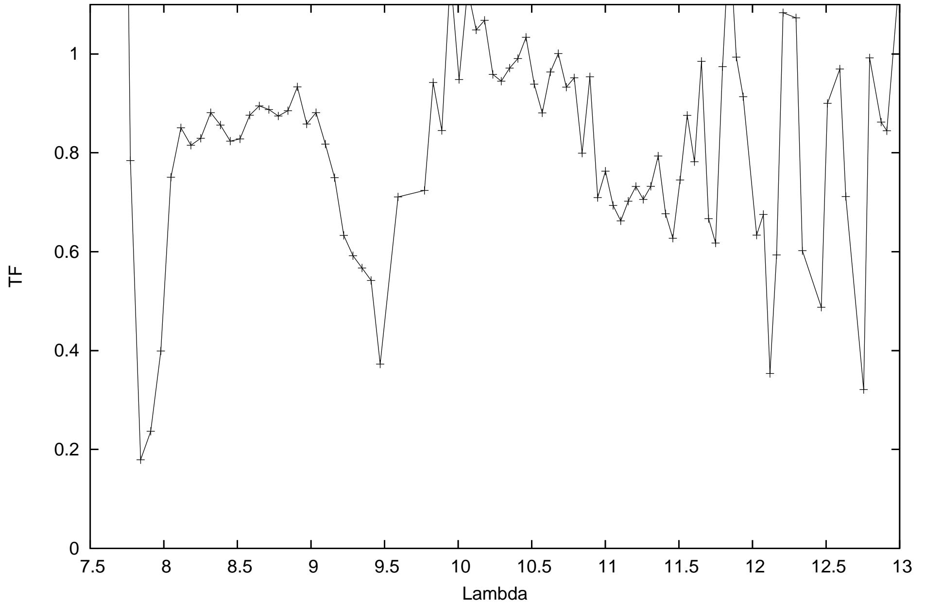
calHIP50371_flux-0.22962_diam5.18_r.MIDI.2012-01-29T02_41_14.970_D0B2
