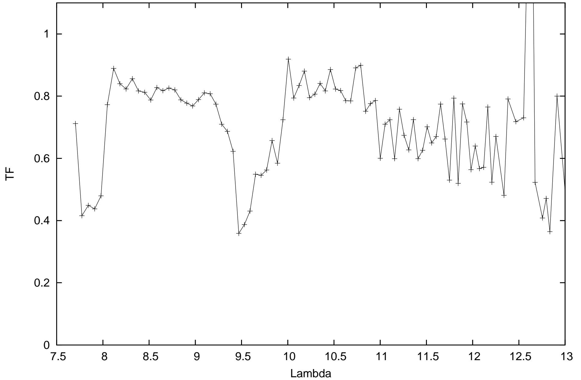
calHIP50371_flux-0.22962_diam5.18_r.MIDI.2012-01-29T06_10_37.127_D0B2
