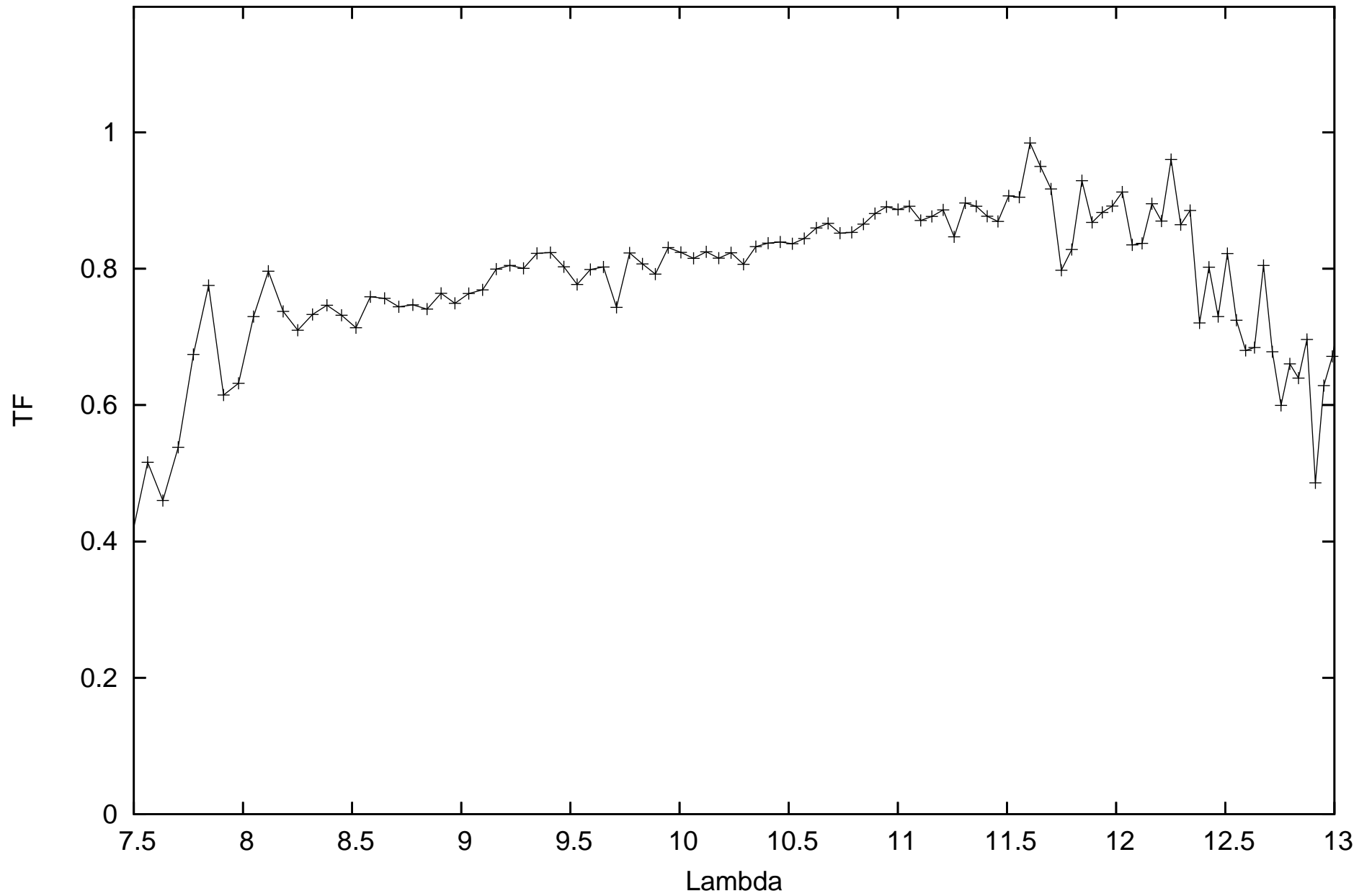
calHD81797_flux-1.49_diam9.14_r.MIDI.2012-02-12T05_08_52.293_C1A1
