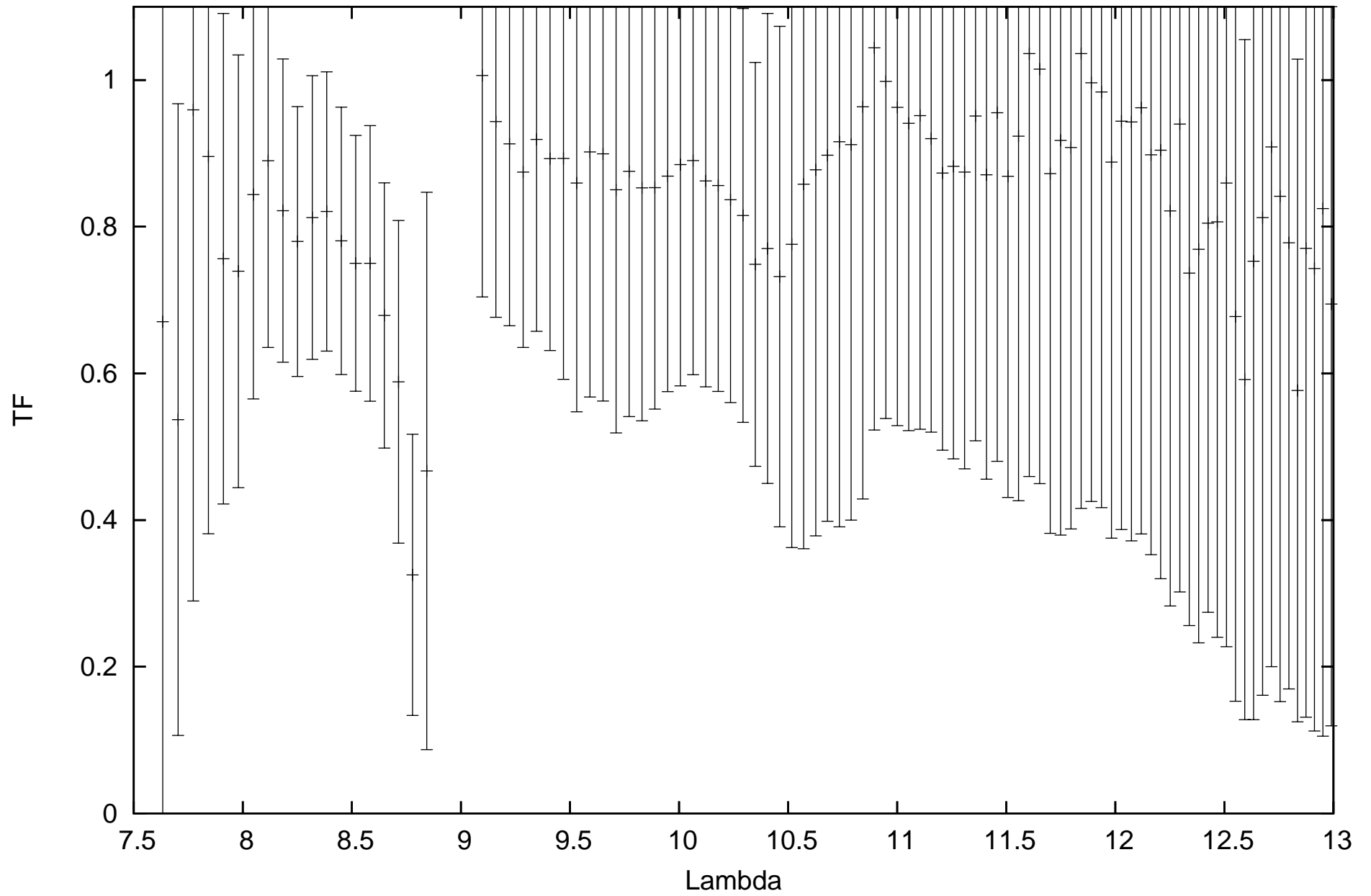
calHD48915_flux-1.39_diam6.09_r.MIDI.2012-02-18T00_50_40.113_C1A1
