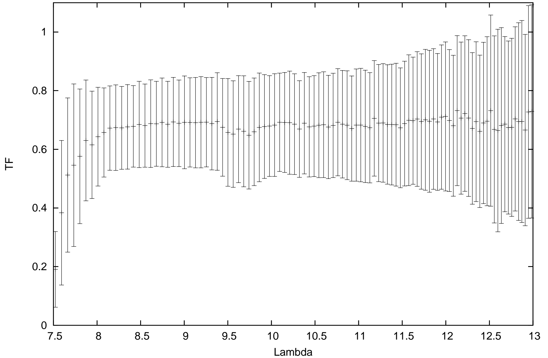
calHD81797_flux-1.49_diam9.14_r.MIDI.2012-02-20T06_04_14.000_D011
