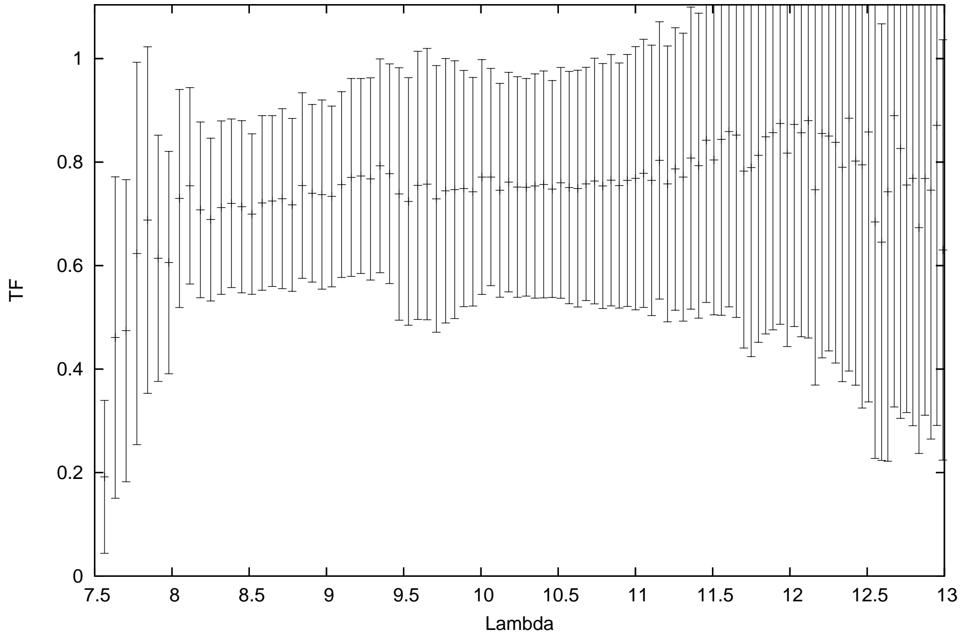
calHD81797_flux-1.49_diam9.14_r.MIDI.2012-02-20T06_12_57.113_D011
