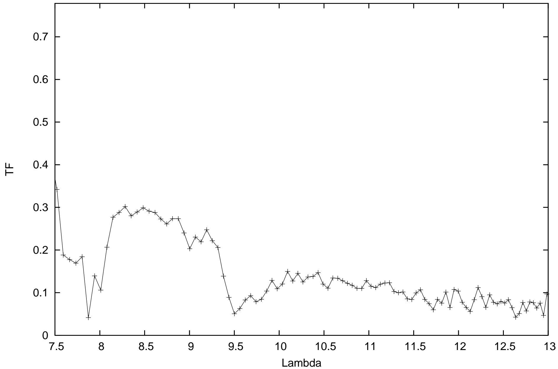
calHD107446_flux0.22_diam4.43_r.MIDI.2012-03-27T07_40_24.000_K011
