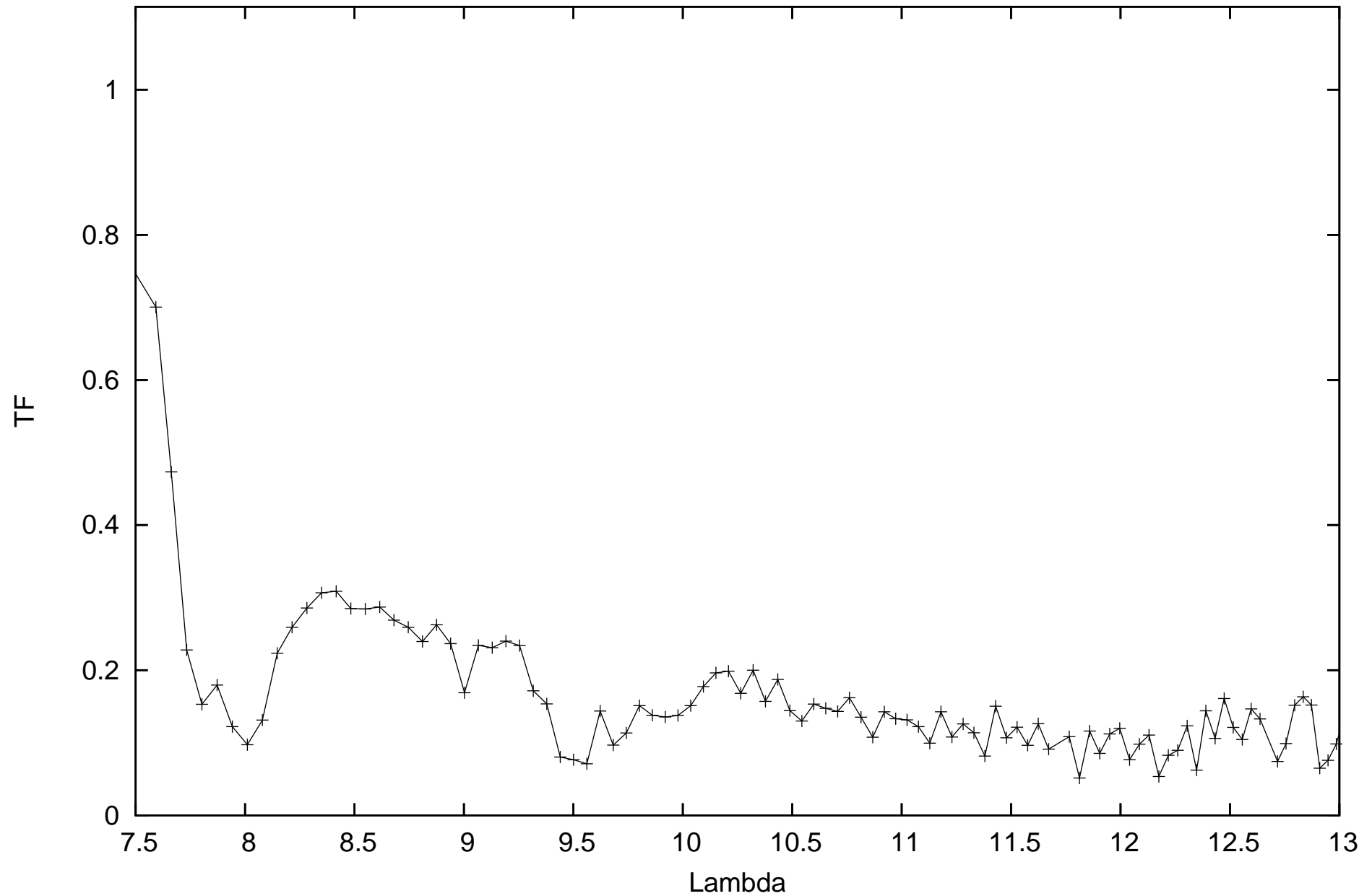
calHD107446_flux0.22_diam4.43_r.MIDI.2012-03-27T08_50_59.000_K0G1
