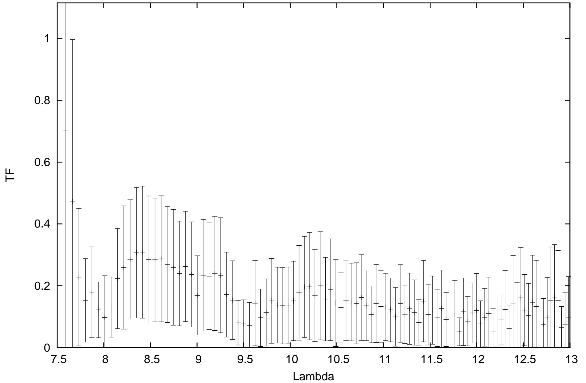
calHD107446_flux0.22_diam4.43_r.MIDI.2012-03-27T08_50_59.000_K0G1
