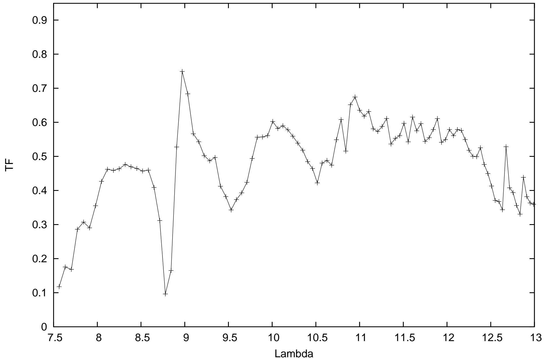
calHD81797_flux-1.49_diam9.14_r.MIDI.2012-04-02T03_58_47.112_K0A1
