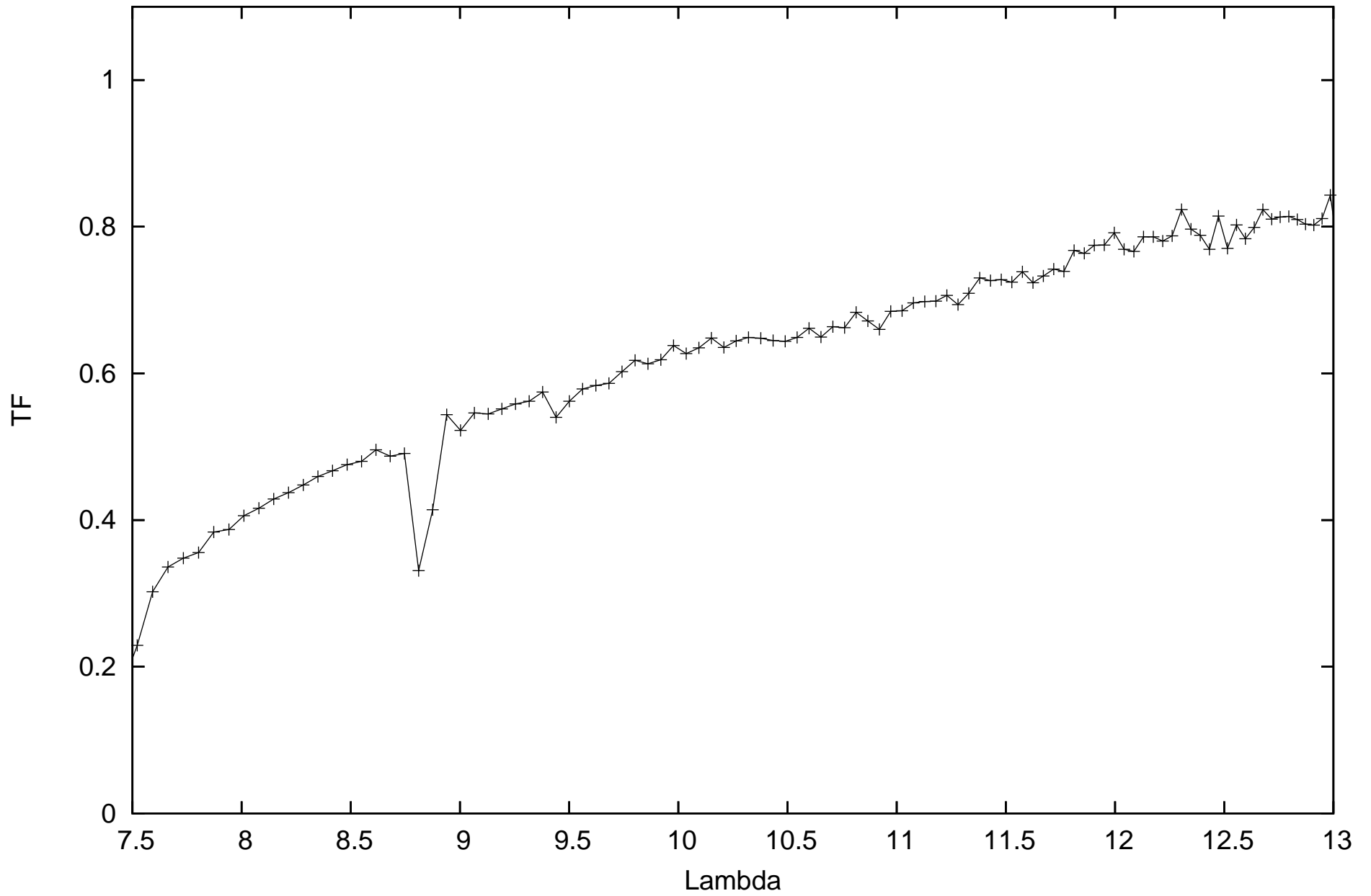
calHIP73714_flux-1.78451_diam11.15_r.MIDI.2012-04-02T05_07_13.000_K0G1
