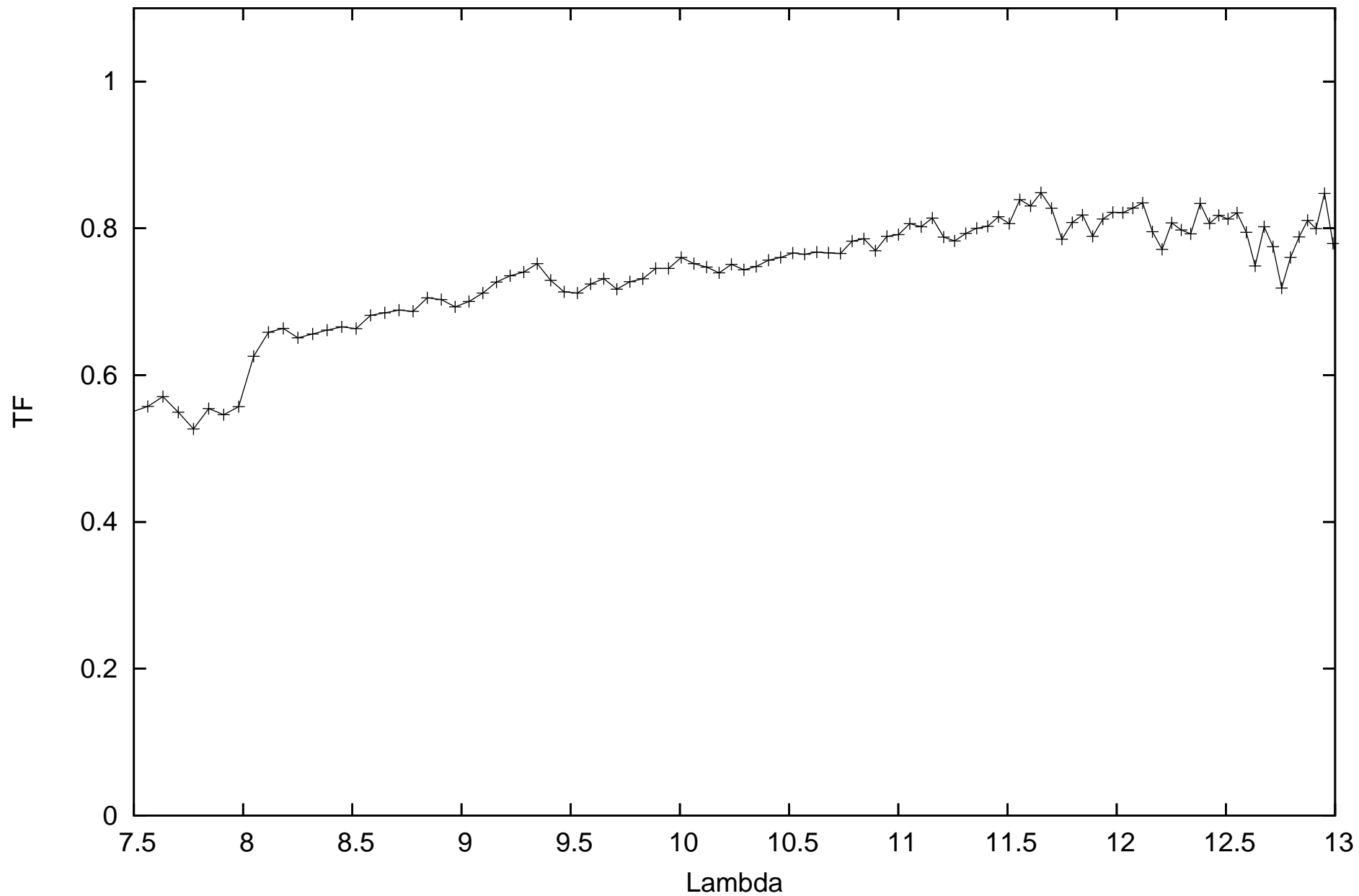
calHD152980_flux0.64_diam3.62_r.MIDI.2012-05-08T09_27_05.969_U3U4
