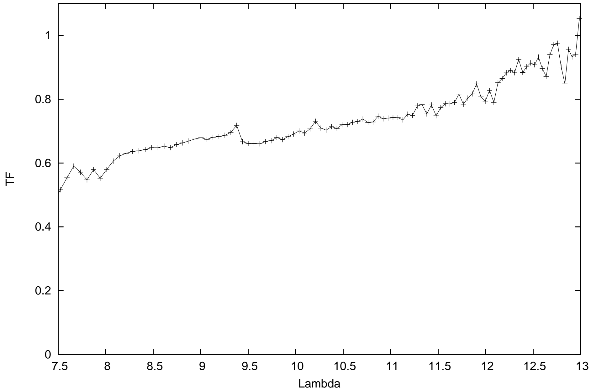
calHIP83081_flux-0.81238_diam6.88_r.MIDI.2012-06-24T05_36_59.000_H011
