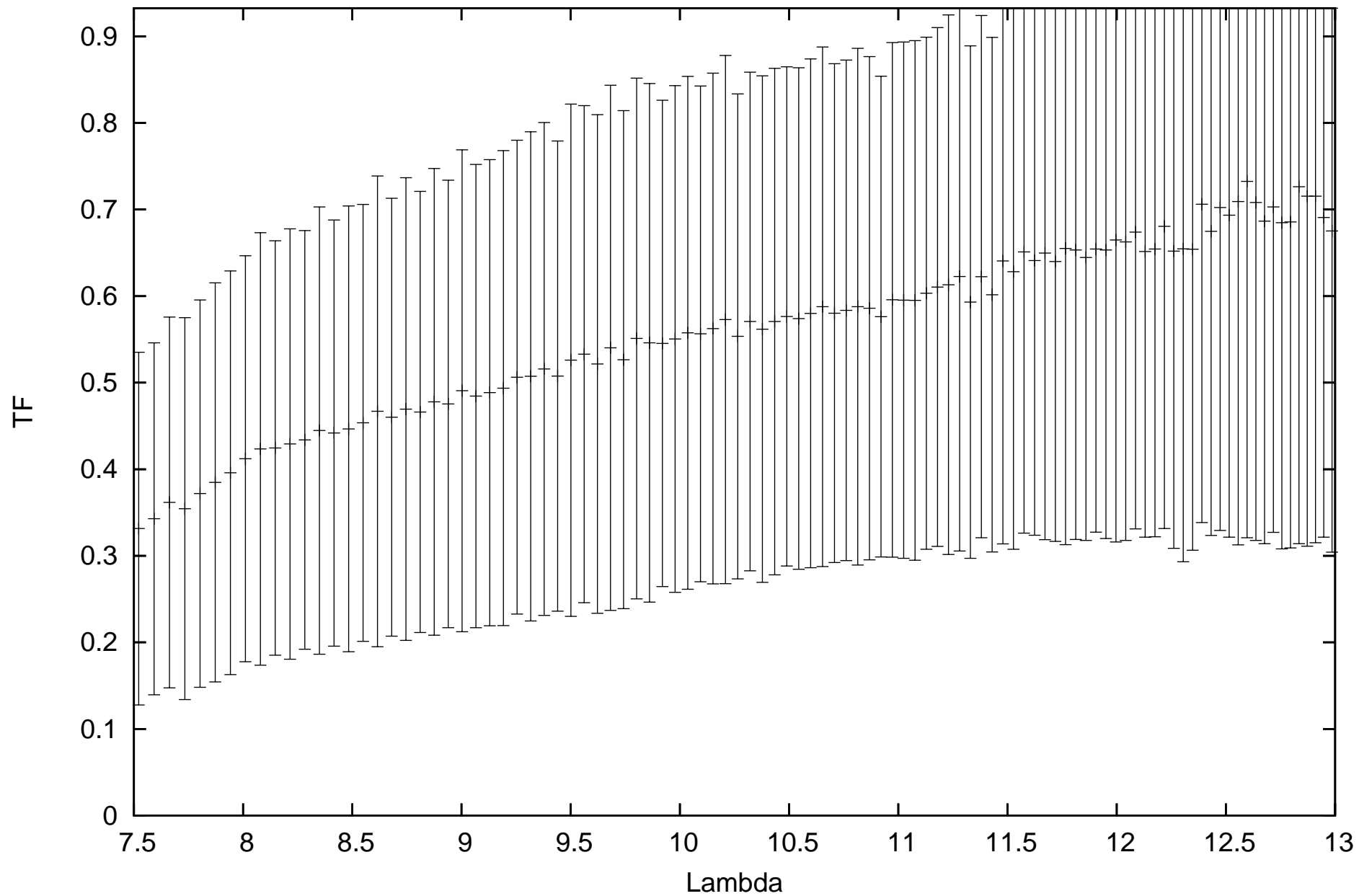
calHD20720_flux-1.53_diam10.14_r.MIDI.2012-07-29T08_38_37.000_C1A1
