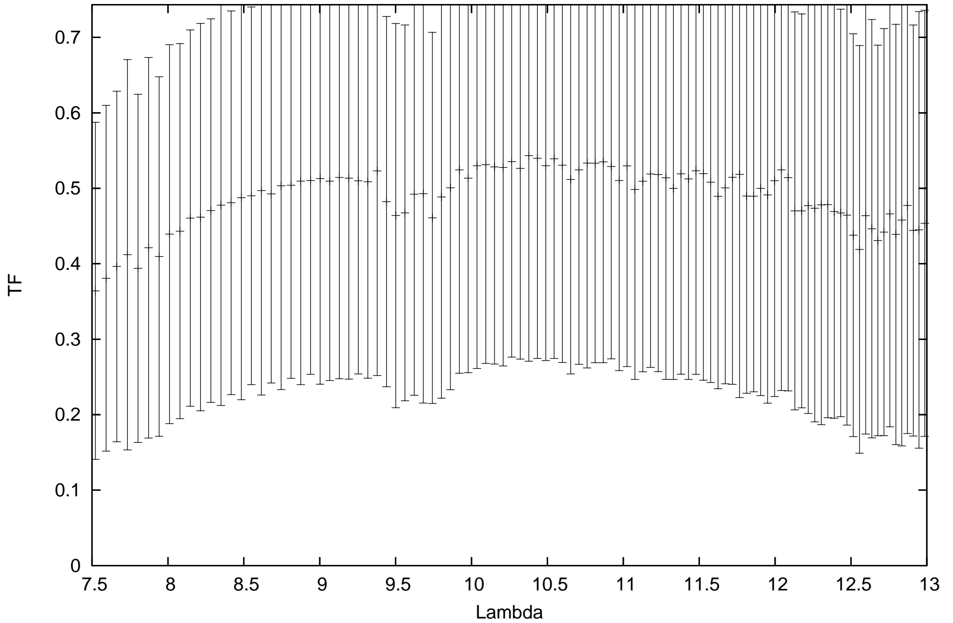
calHD224935_flux-0.85_diam7.24_r.MIDI.2012-07-29T08_17_20.000_C1A1
