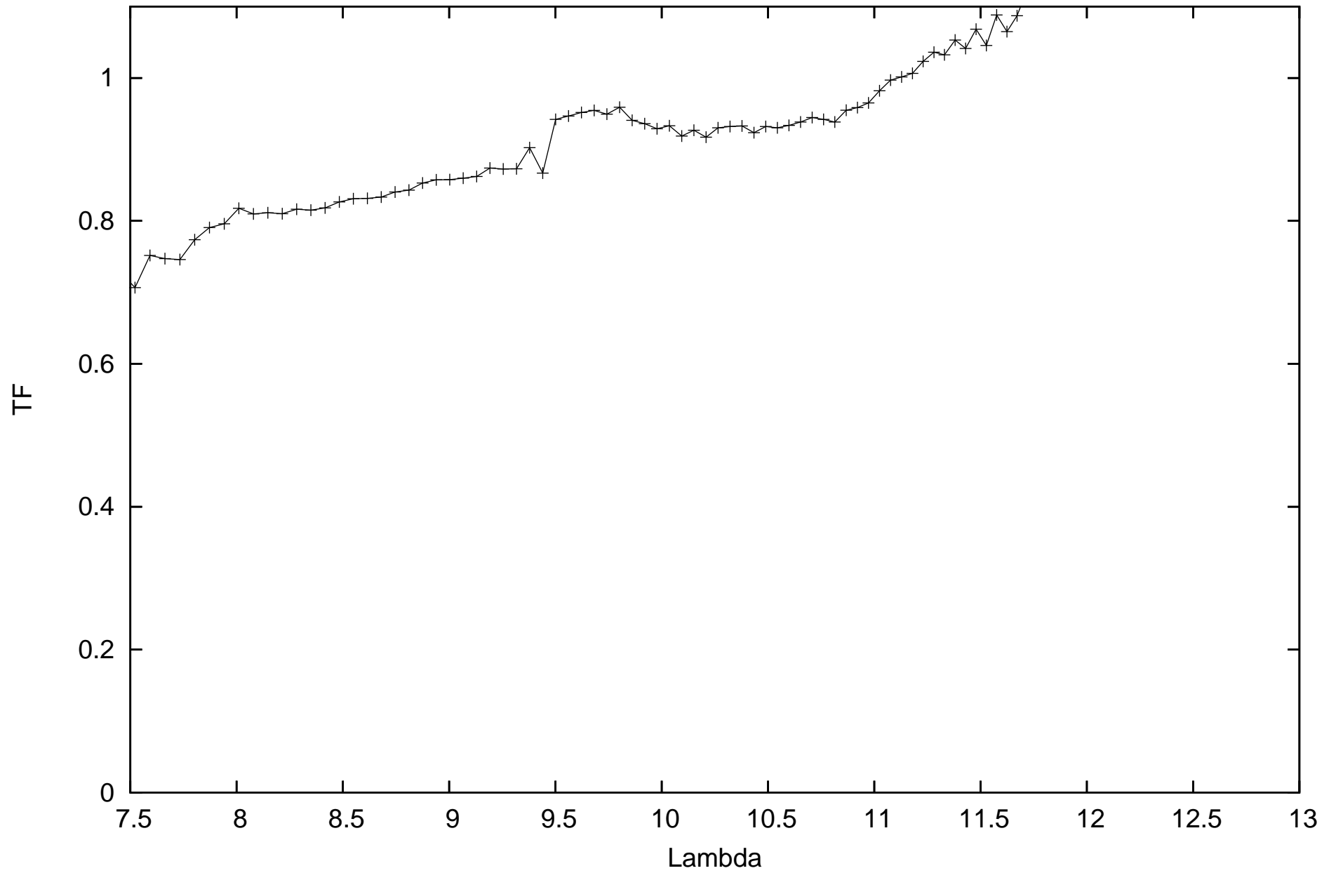
calHD167618_flux-1.82_diam11.66_r.MIDI.2012-09-22T02_42_05.000_C1B2
