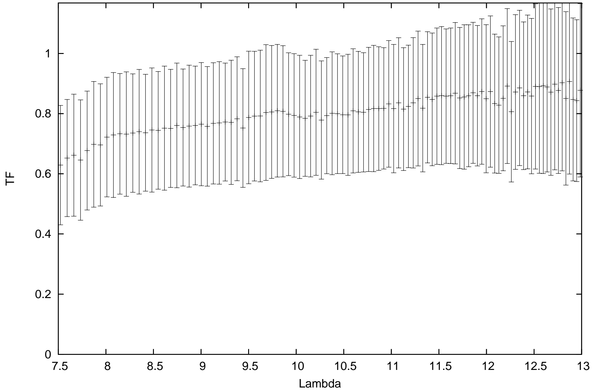
calHD167618_flux-1.82_diam11.66_r.MIDI.2012-09-26T01_48_19.000_C1A1
