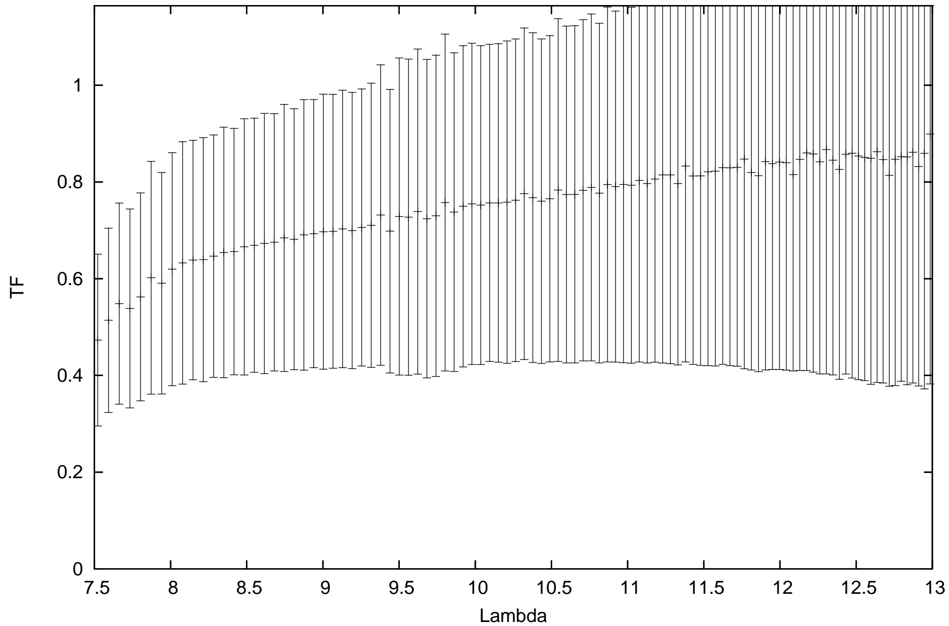
calHIP14135_flux-1.95419_diam12.27_r.MIDI.2012-10-05T07_14_39.000_K0J3
