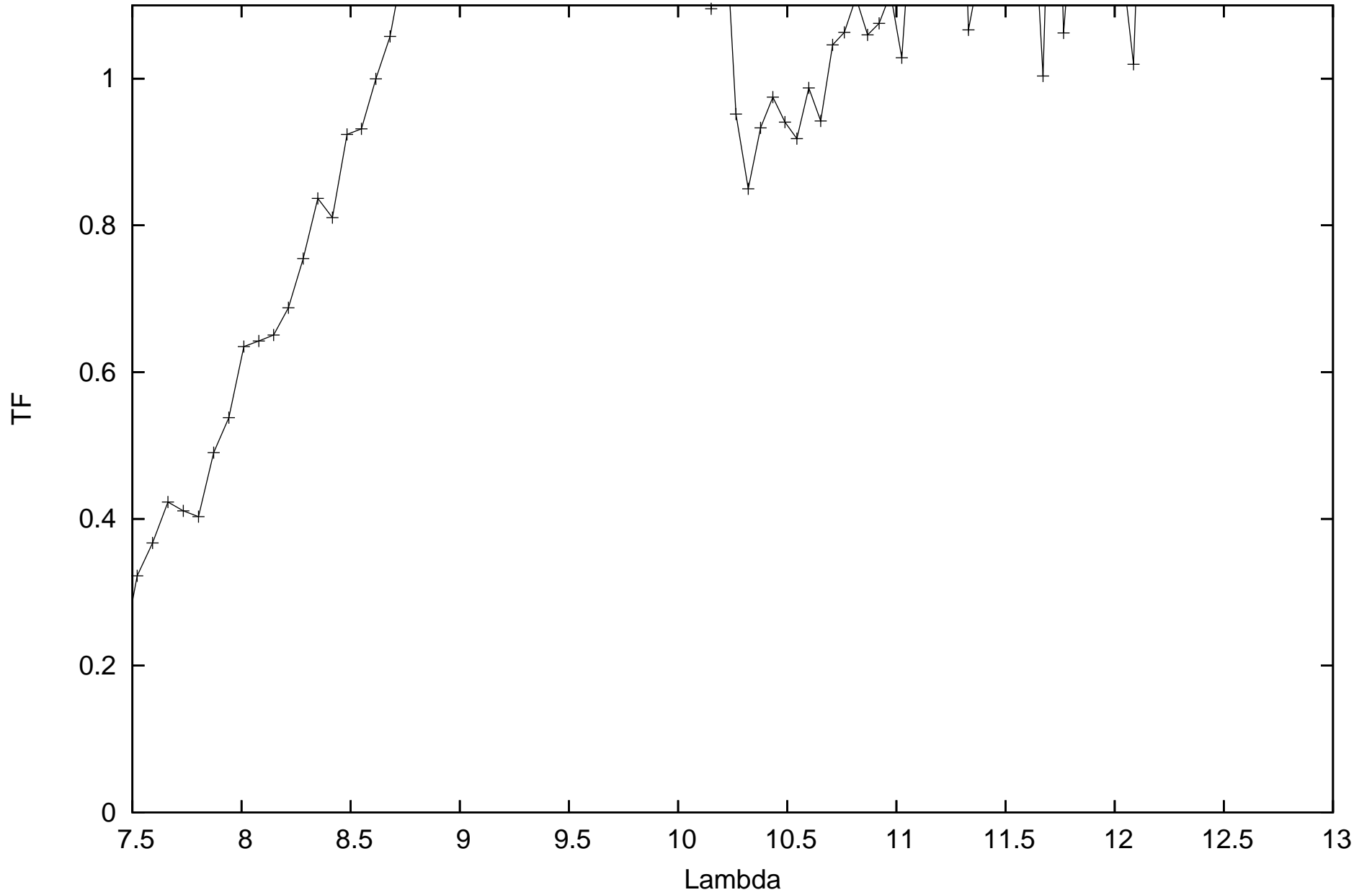
calHIP23685_flux-0.41239_diam5.994598_r.MIDI.2012-10-12T04_34_07.000_A1G1
