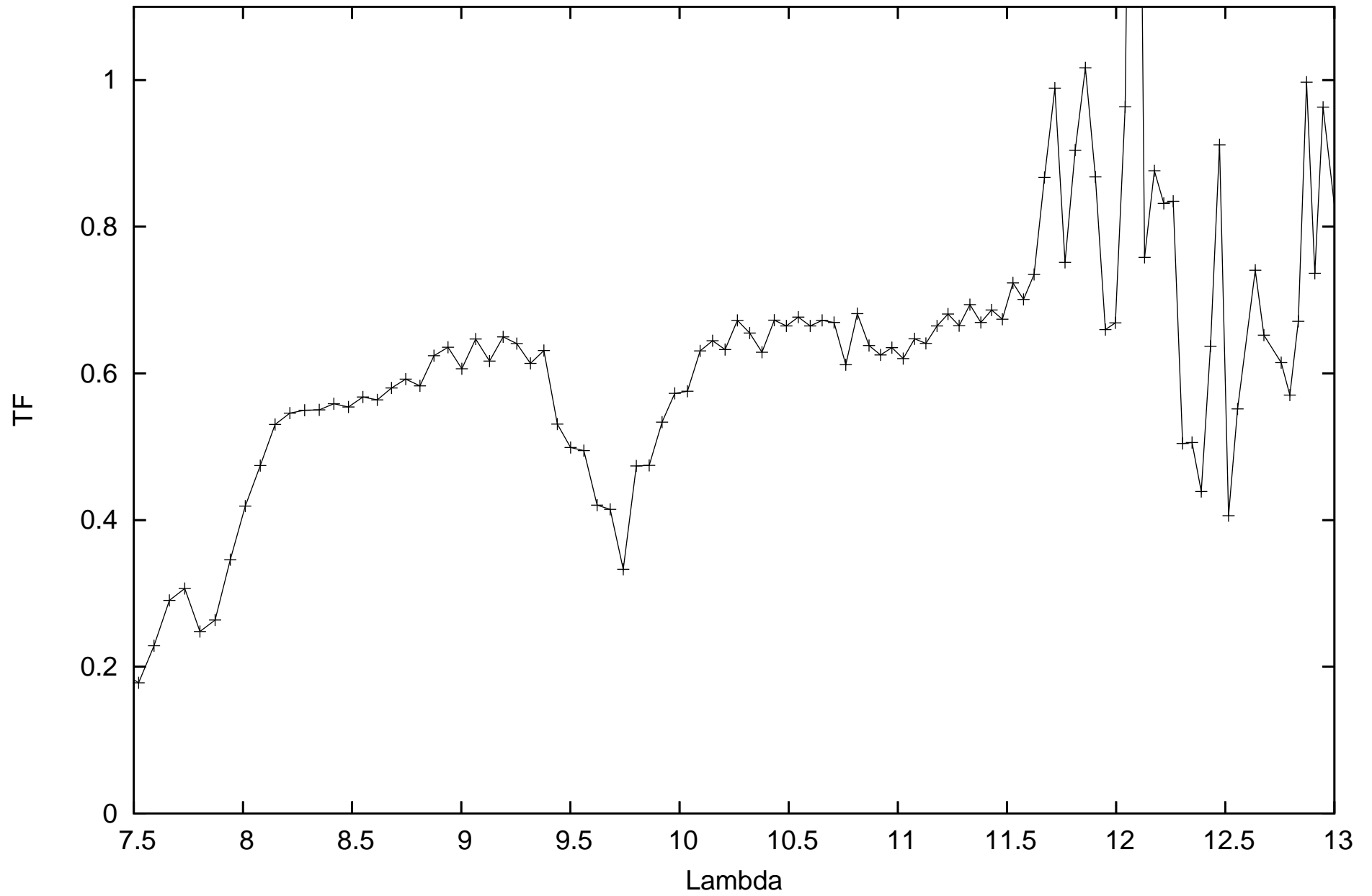
calHD1014_flux0.24_diam4.61_r.MIDI.2012-10-04T07_17_47.000_A1J3
