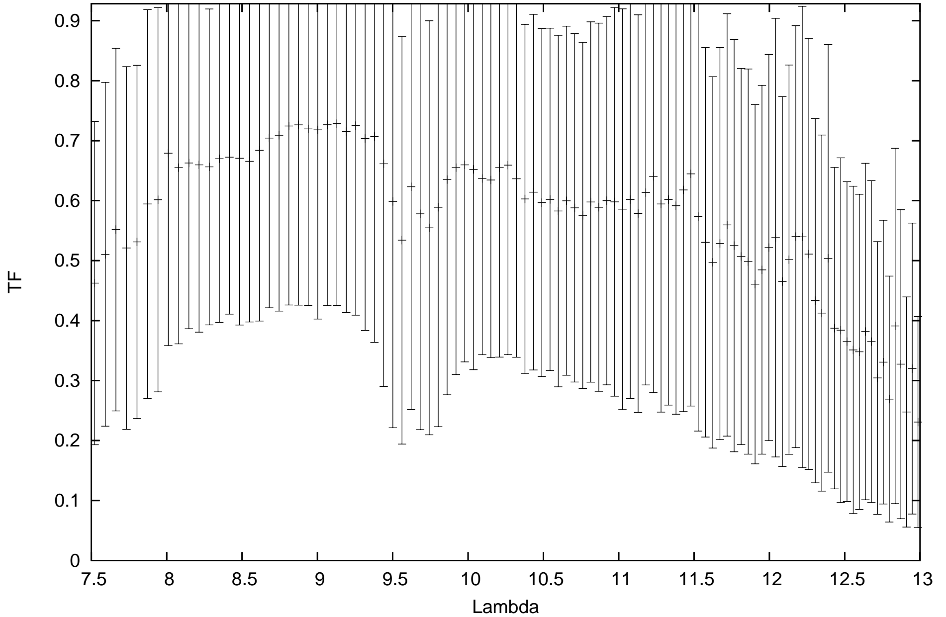
calHD1014_flux0.24_diam4.61_r.MIDI.2012-11-18T01_04_52.000_D0H0
